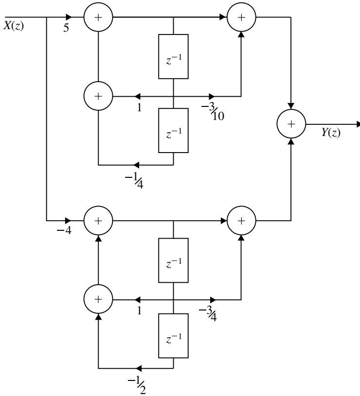
Fig. 4.51 Parallel form realization of H(z) for the Example 4.38
