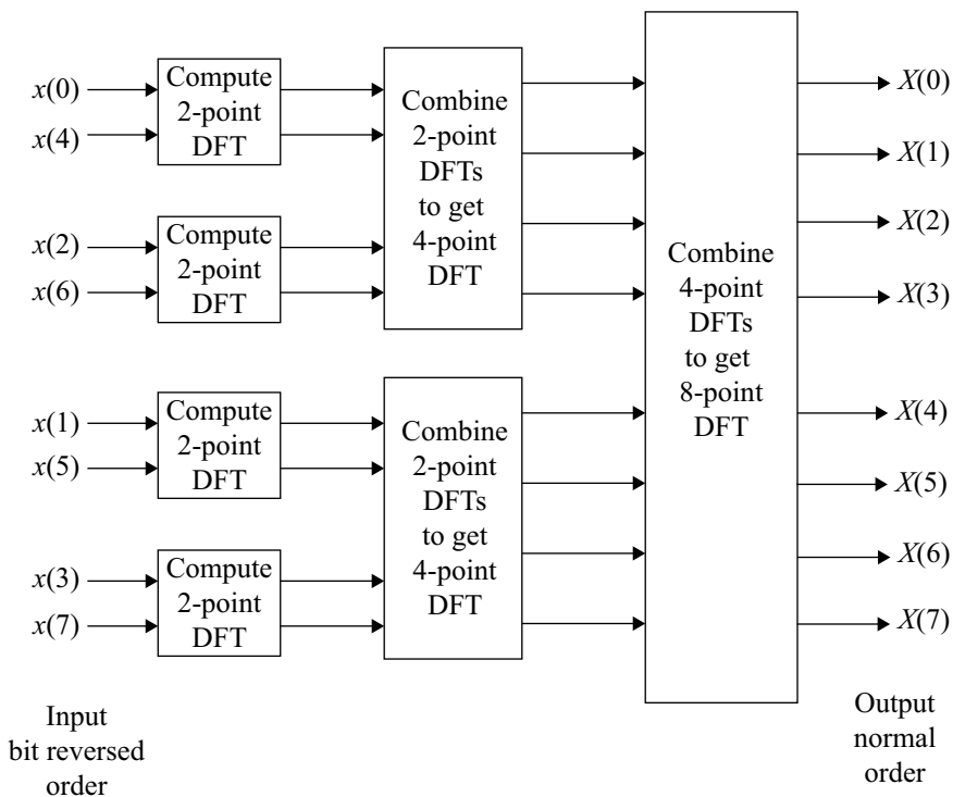
Fig. 3.16 Block diagram of radix-2 DIT FFT
