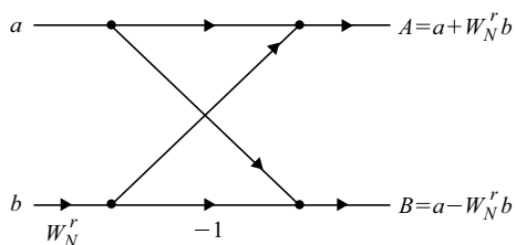
Fig. 3.15 Basic butterfly computation in the DIT FFT algorithm
