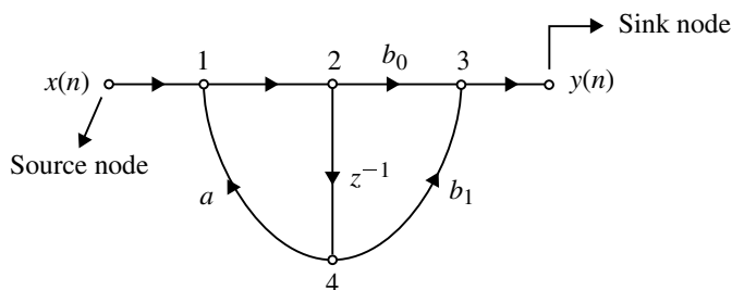
Fig. 4.35 Signal flow graph of first order system
