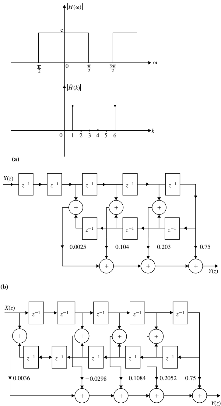
Fig. 5.40 Magnitude response for Example 5.23. a Structure realization for Example 5.24. b Structure realization for Example 5.24
