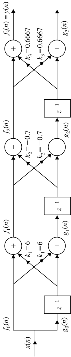
Fig. 5.15 Lattice structure for Example 5.6
