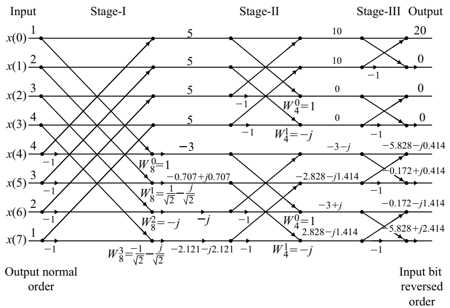
Fig. 3.30 Butterfly diagram of Example 3.33(ii)
