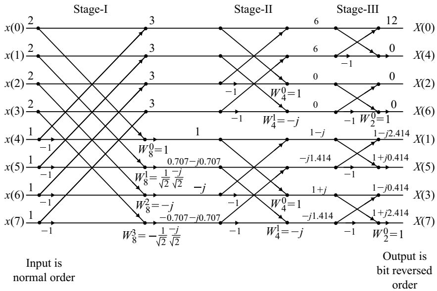
Fig. 3.24 Butterfly diagram of Example 3.31(ii)
