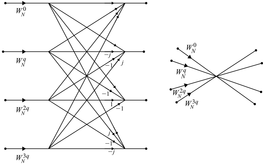
Fig. 3.22 Basic butterfly in a radix-4 FFT algorithm
