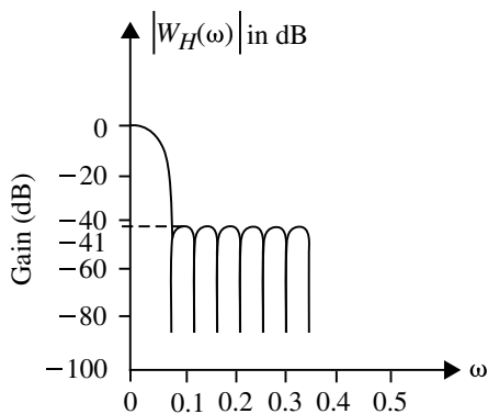
Fig. 5.50 Log-magnitude spectrum of Hamming window
