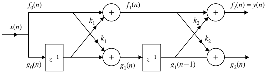
Fig. 5.14 Two-stage all-zero lattice structure
