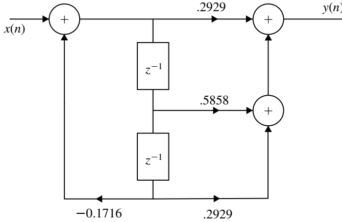
Fig. 4.18 Direct form-II realization of H(z) for the Example 4.10(a)
