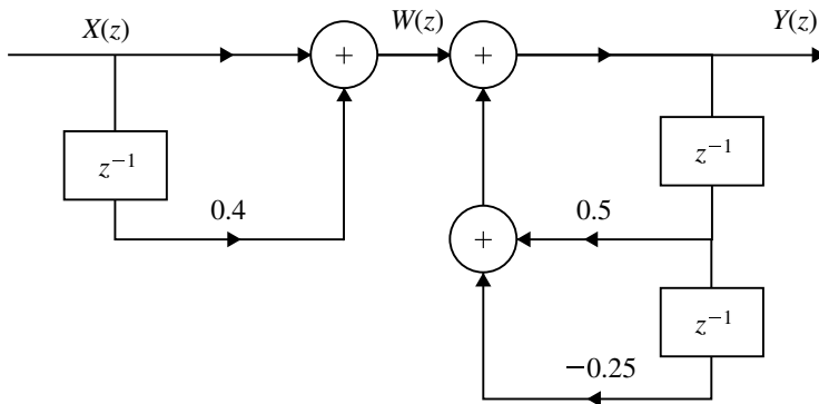
Fig. 4.37 Direct form-I realization for Example 4.30
