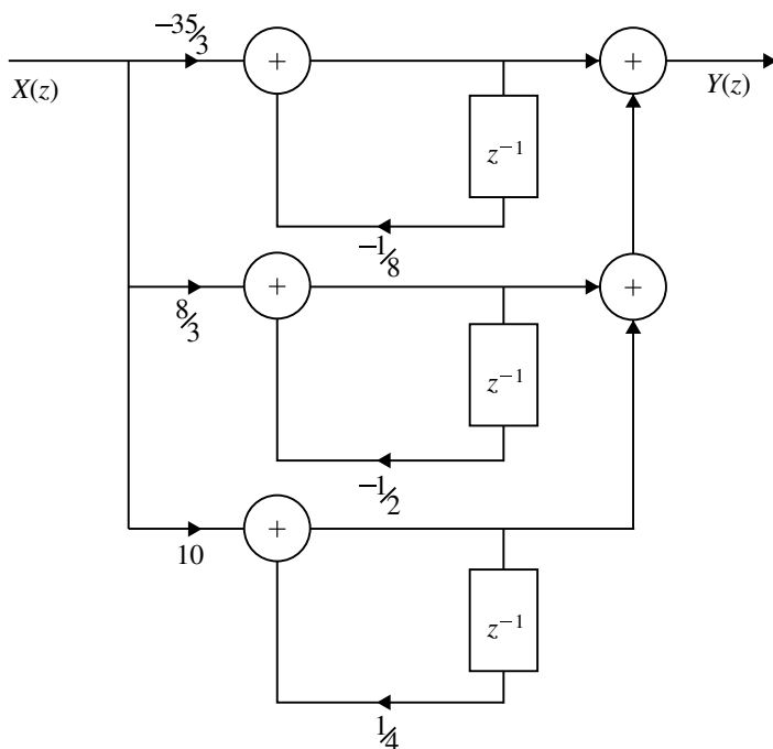
Fig. 4.49 Parallel form realization of H(z) for the Example 4.37
