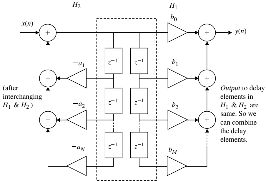
Fig. 4.31 Conversion of Direct form-I to Direct form-II structure
