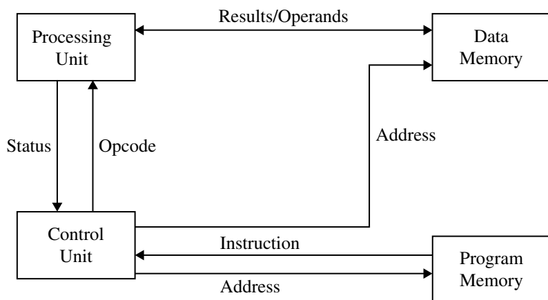
Fig. 6.3 Harvard architecture
