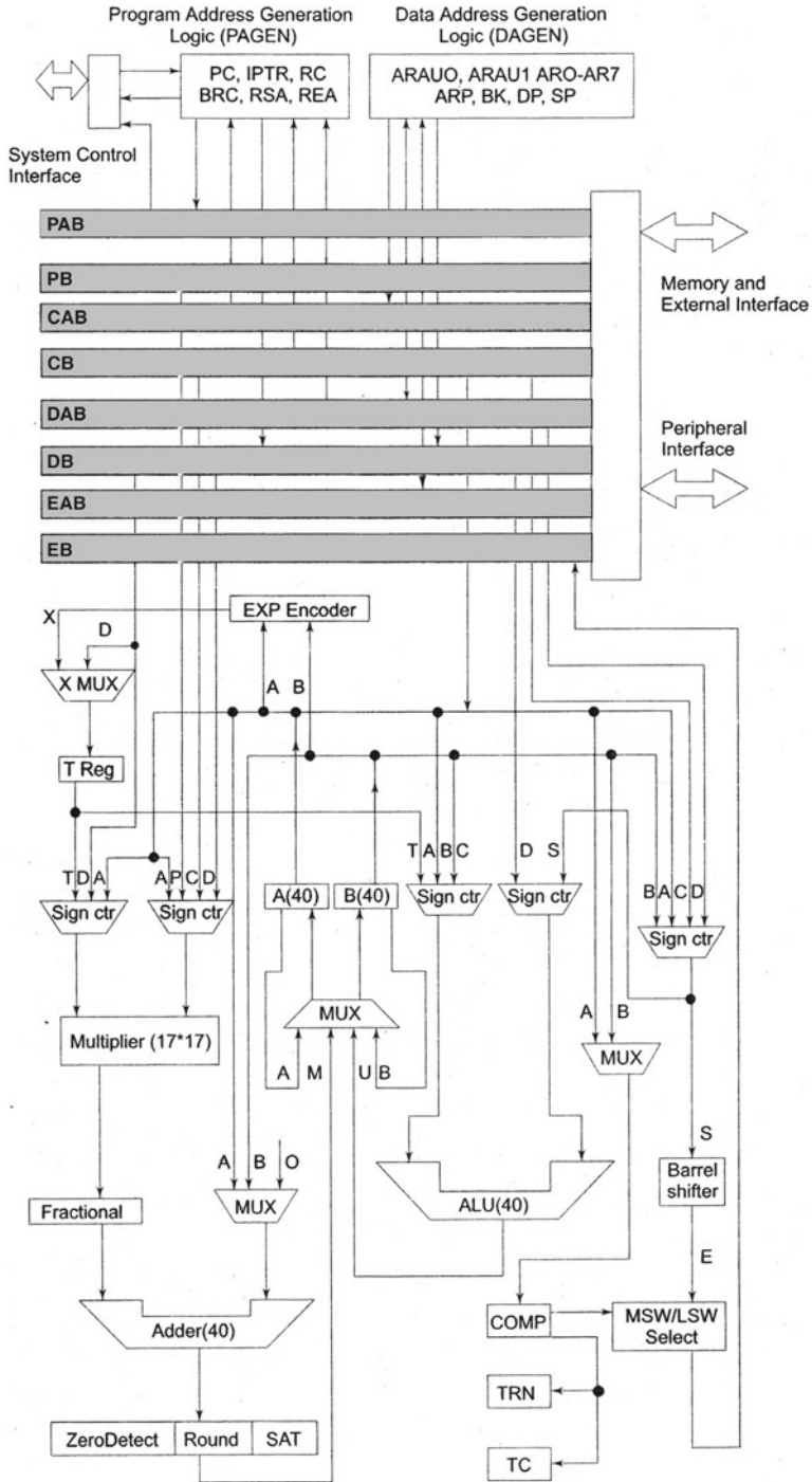
Fig. 6.12 Block diagram of 54x internal hardware
