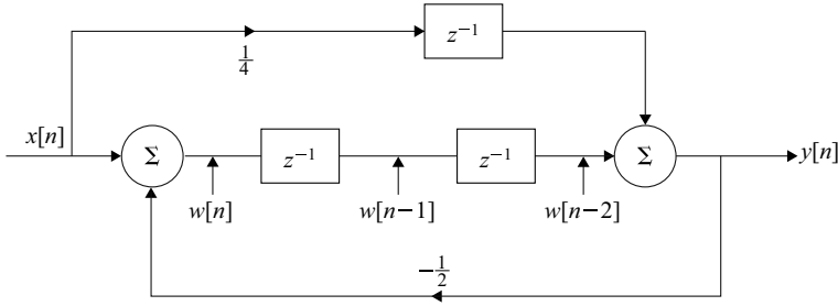
Fig. 2.18 Block diagram of Example 2.42
