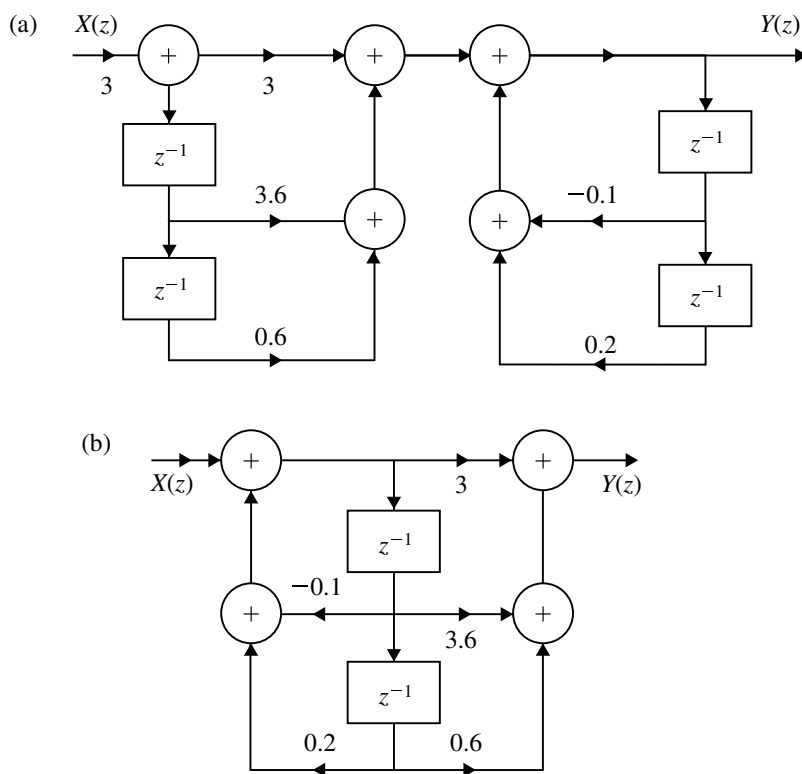
Fig. 4.41 a, b Direct form-I and form-II realization for Example 4.34
