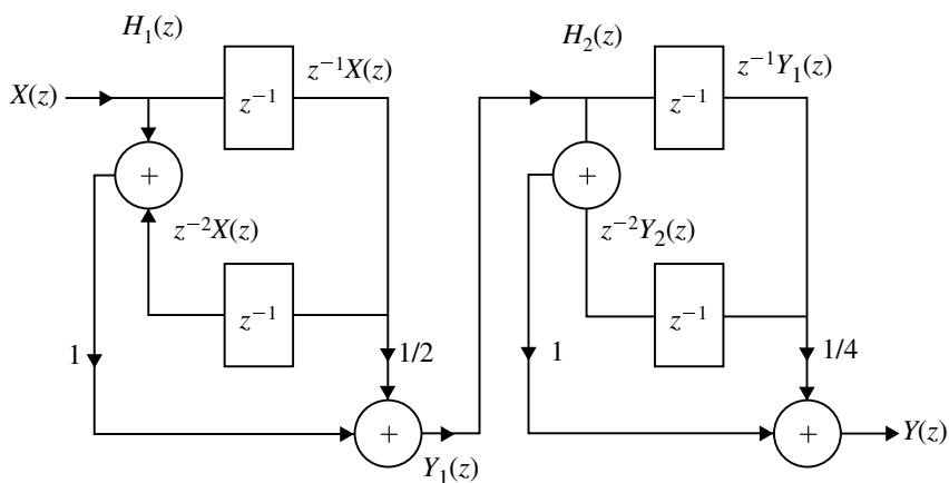
Fig. 5.12 Linear phase realization of H(z) for Example 5.4(iii)
