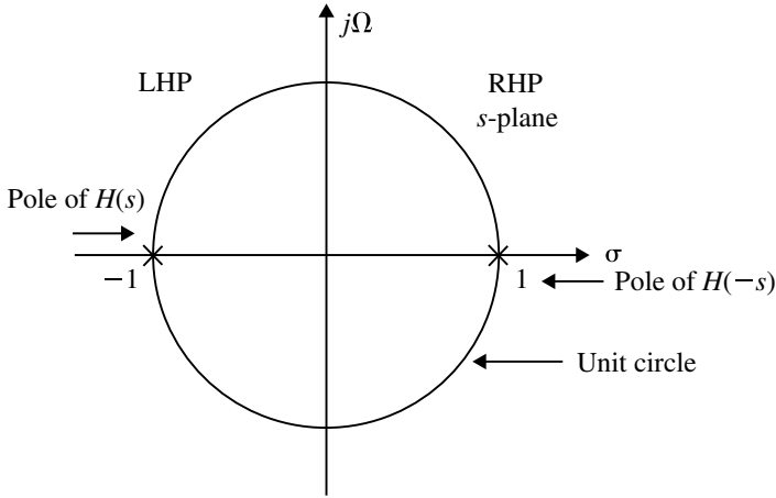
Fig. 4.11 Pole location of first order filter
