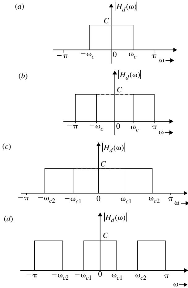
Fig. 5.1 Magnitude response of ideal lowpass, highpass, bandpass and bandstop filter
