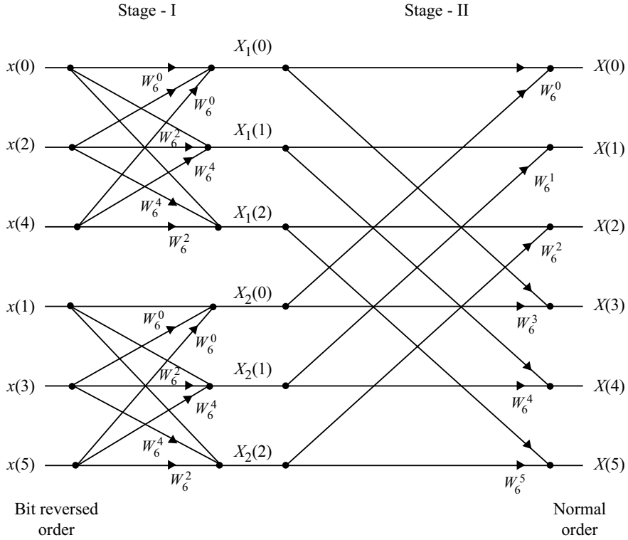
Fig. 3.41 DIT FFT flow diagram for N = 6 = 2 \cdot 3
