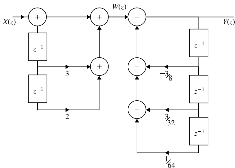
Fig. 4.46 Direct form-I realization of H(z) for the Example 4.37
