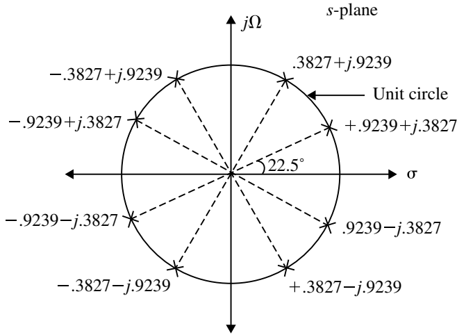
Fig. 4.14 Pole location of fourth order filter
