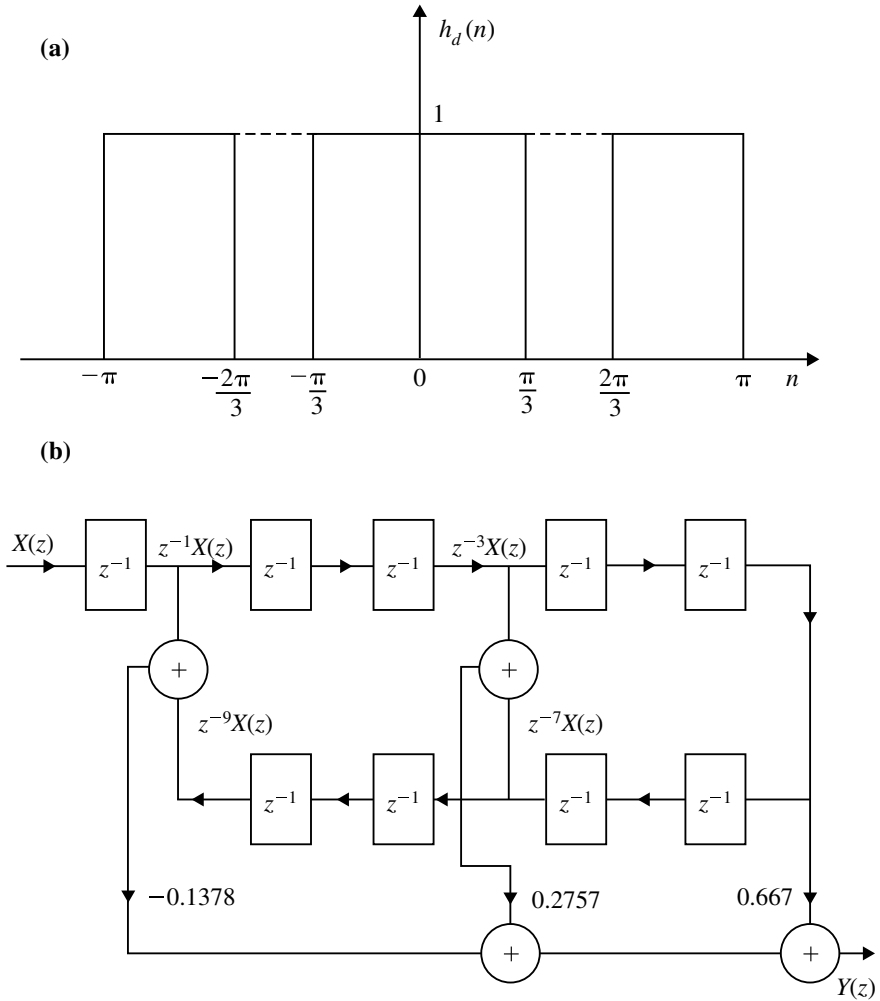
Fig. 5.29 a Impulse response for 5.12. b Structure realization for Example 5.12
