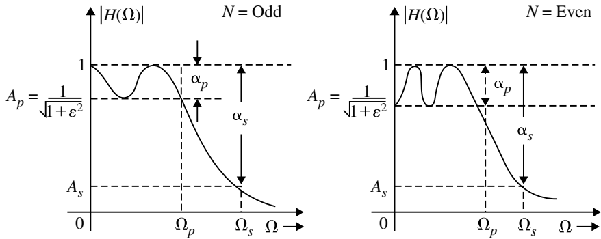
Fig. 4.21 Frequency response of type I Chebyshev filter
