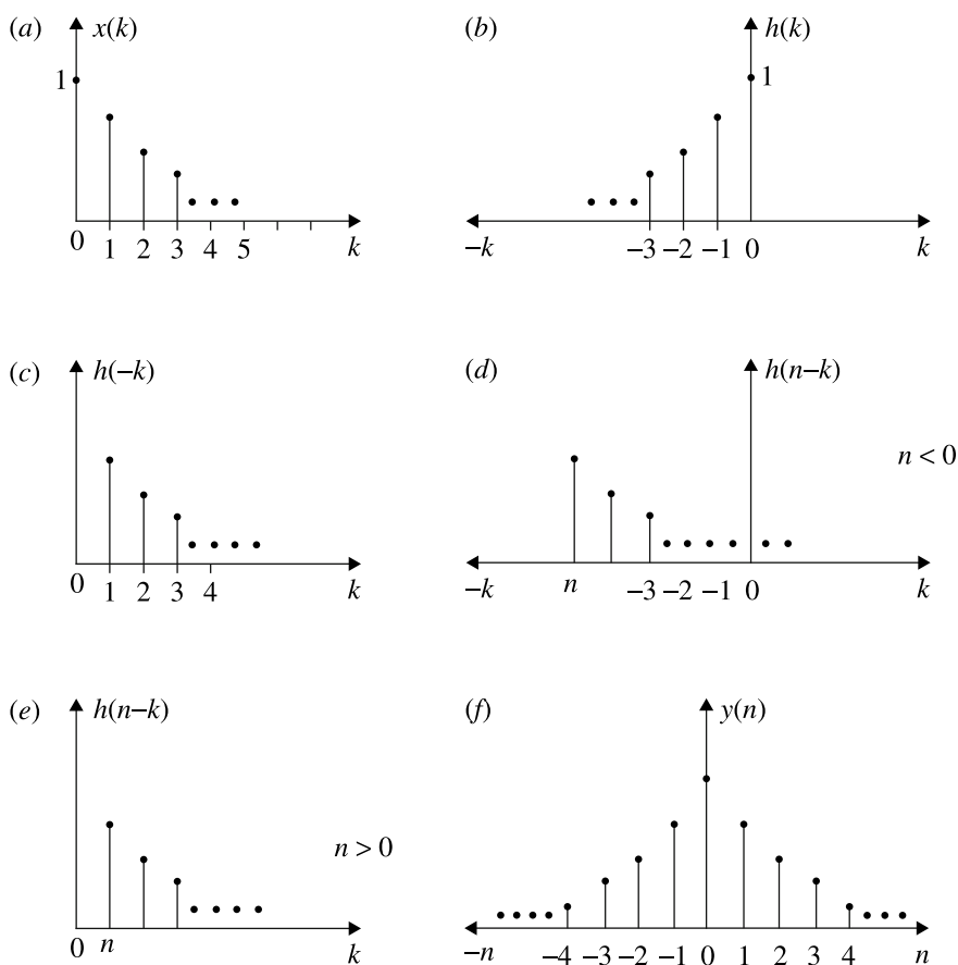
Fig. 2.29 Convolution of casual and anti-causal signals
