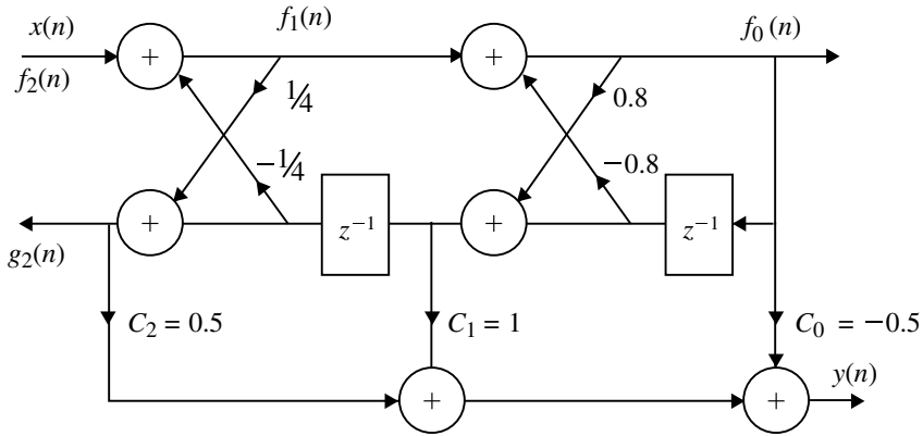
Fig. 4.60 Lattice-Ladder form for the Example 4.42
