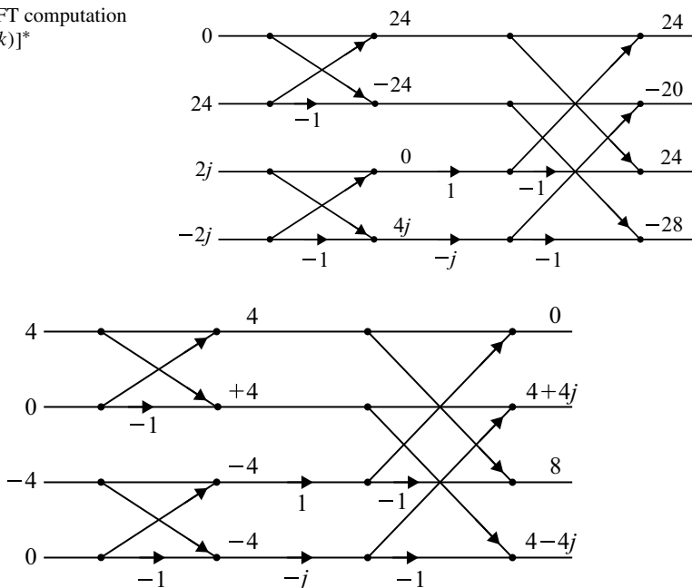
Fig. 3.61 DFT Computation of x_3(k)
