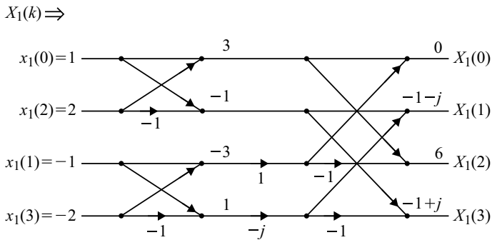
Fig. 3.56 Butterfly diagram of X_1(k)
