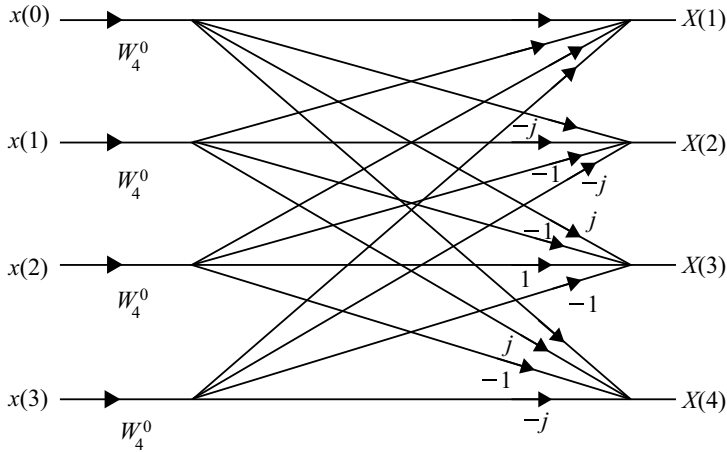
Fig. 3.21 4-Point radix-4 FFT butterfly diagram
