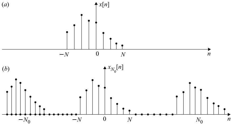
Fig. 2.19 Extension of aperiodic signal to periodic signal
