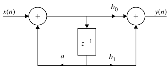
Fig. 4.34 First order system
