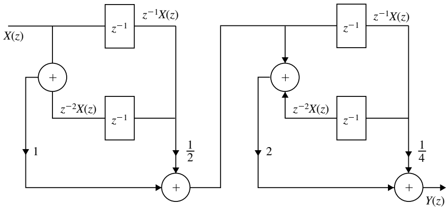
Fig. 5.9 Cascade connection of linear phase FIR filter of Example 5.3
