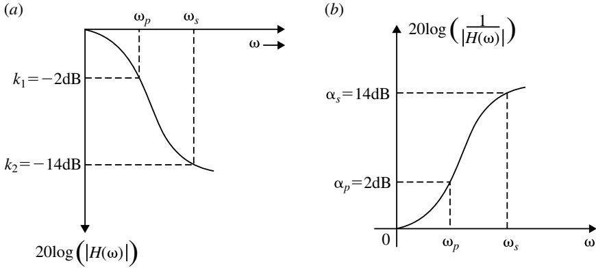
Fig. 4.9 Gain and attenuation V_s\omega in dB
