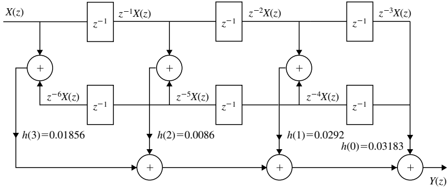
Fig. 5.44 Realization of FIR filter for Example 5.28
