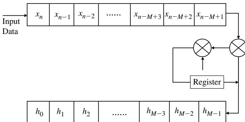
Fig. 6.1 Implementation of convolution with array multiplier (Single multiplier/Adder)
