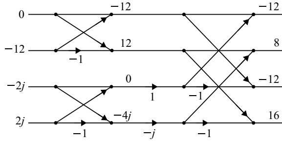
Fig. 3.58 Butterfly diagram of [X_1(k)H(k)]^*
