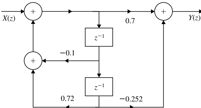
Fig. 4.39 Direct form-II realization for Example 4.32
