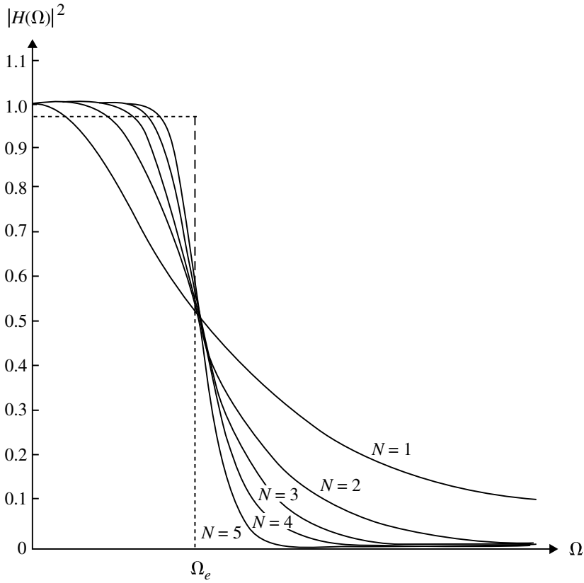
Fig. 4.15 Frequency response of Butterworth filter
