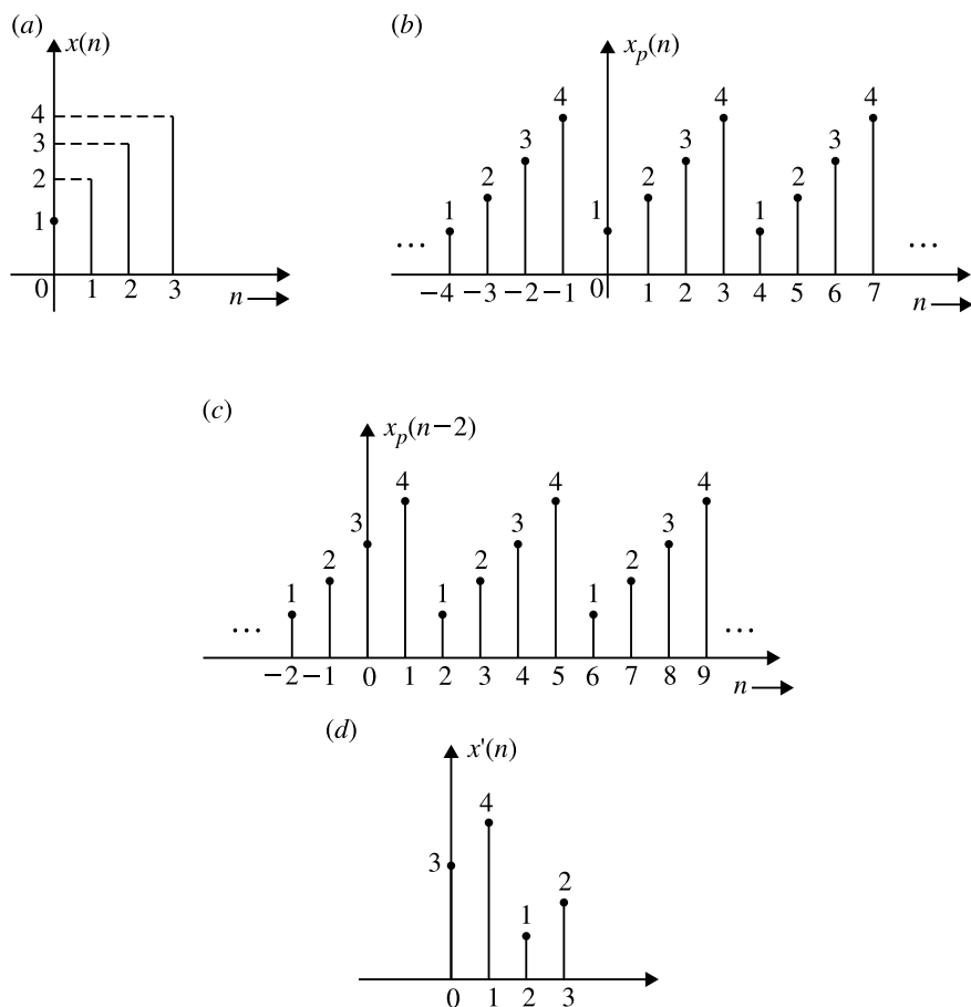
Fig. 3.9 a Discrete time signal x(n) , b periodic extension of x(n) , c shifted periodic extension of x(n) and d Discrete time signal x'(n)
