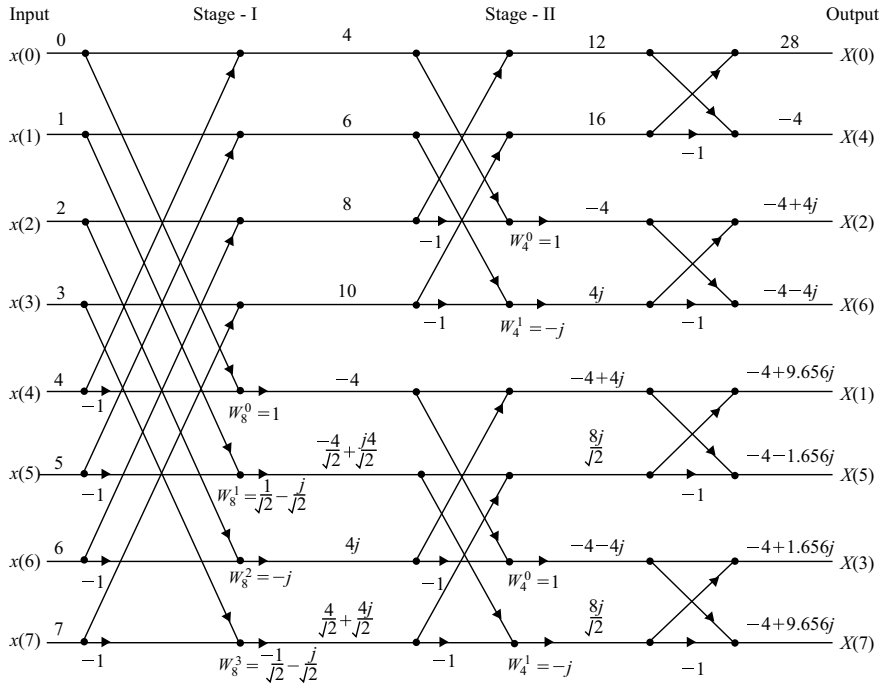
Fig. 3.38 Butterfly diagram for Example 3.41
