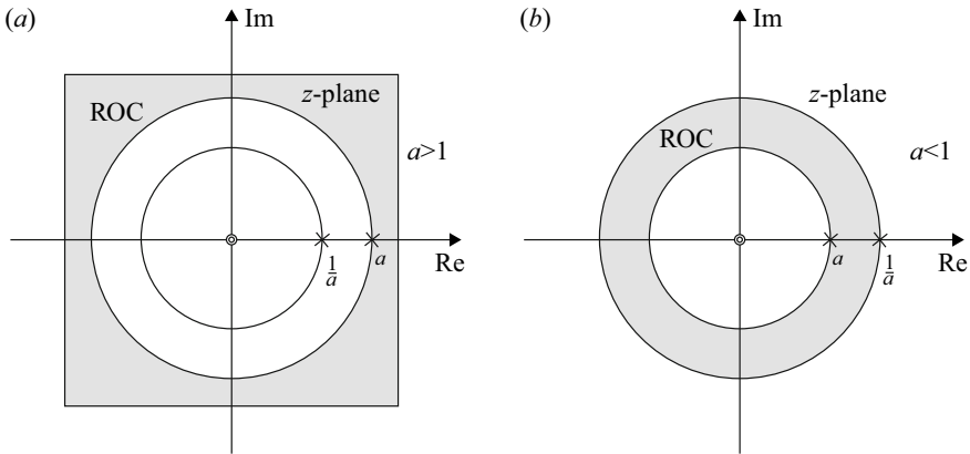
Fig. 2.13 ROC of Example 2.8
