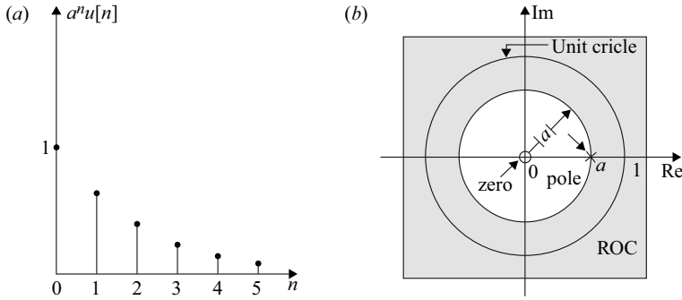
Fig. 2.2 a x[n] = a^n u[n] and b ROC: 0 < a < 1
