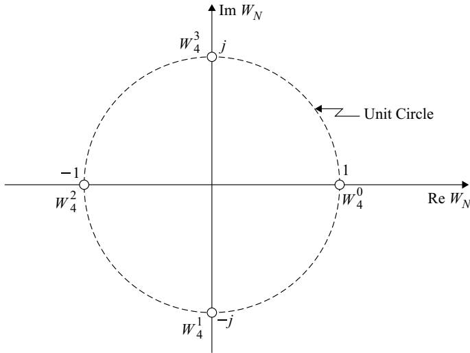
Fig. 3.1 Representation of W_4^{-nk}
