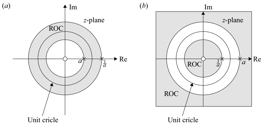
Fig. 2.5 ROC of x[n] = a^{|n|} . a a < 1 and b a > 1
