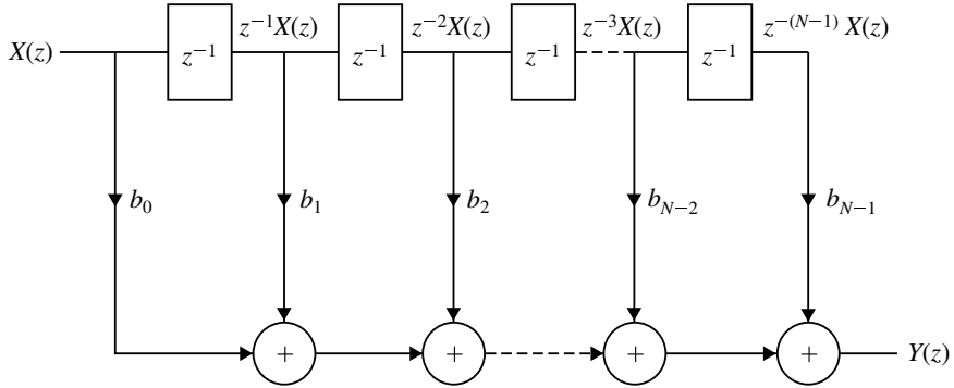
Fig. 5.3 Direct form realization
