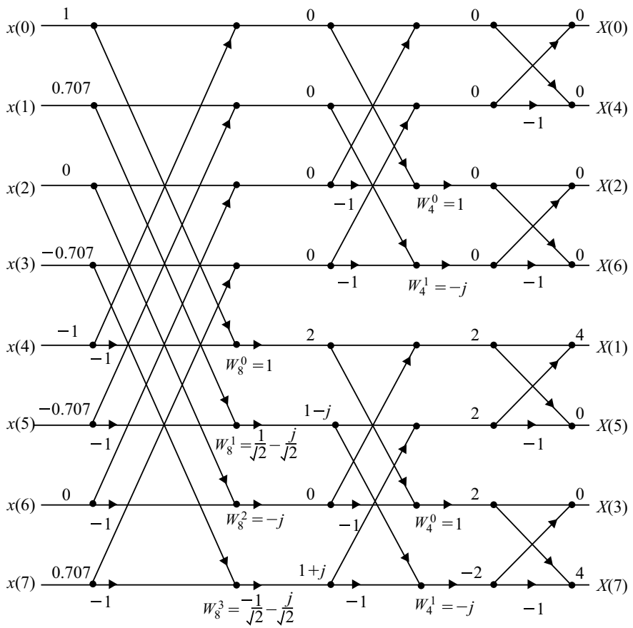
Fig. 3.35 Butterfly diagram for Example 3.38
