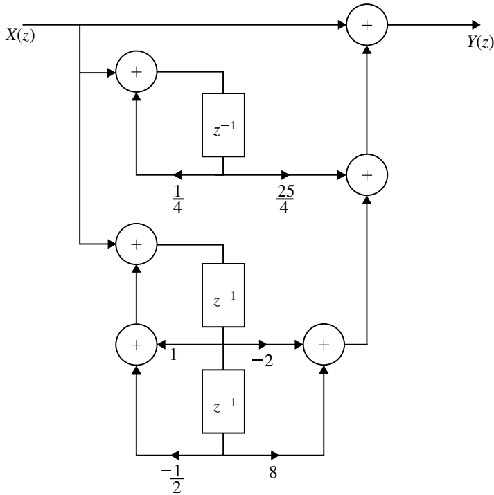
Fig. 4.53 Parallel form realization of H(z) for the Example 4.39
