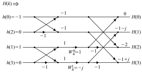
Fig. 3.50 Butterfly diagram of H(k)
