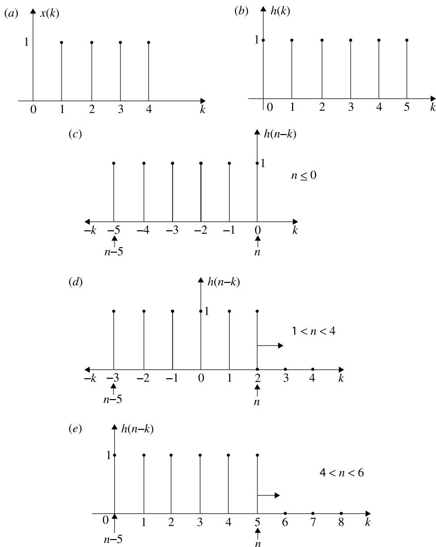
Fig. 2.33 Convolution sum for Example 2.64. Response plot of Example 2.64
