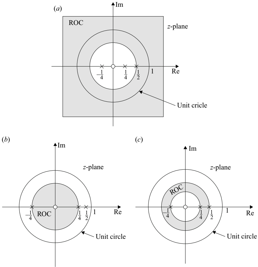
Fig. 2.17 a Pole-zero diagram and ROC: |z| > \frac{1}{2} of Example 2.27. b Pole-zero diagram and ROC: |z| < \frac{1}{4} and c Pole-zero diagram and ROC: \frac{1}{4} < |z| < \frac{1}{2}
