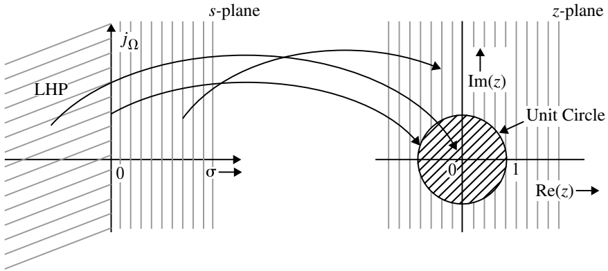
Fig. 4.4 Mapping of s -plane into z -plane in Bilinear transformation
