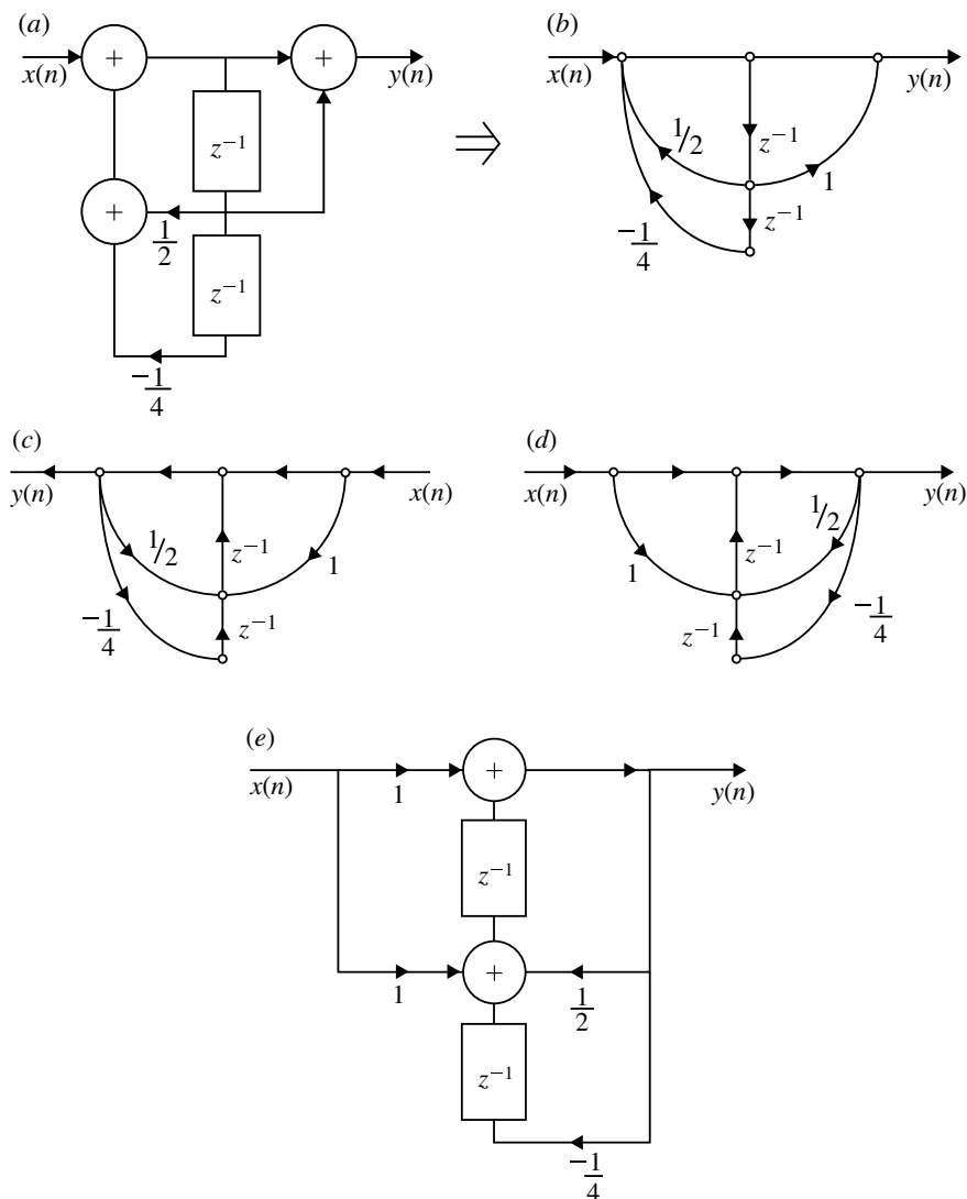
Fig. 4.54 Transposed direct form-II realization for the Example 4.40
