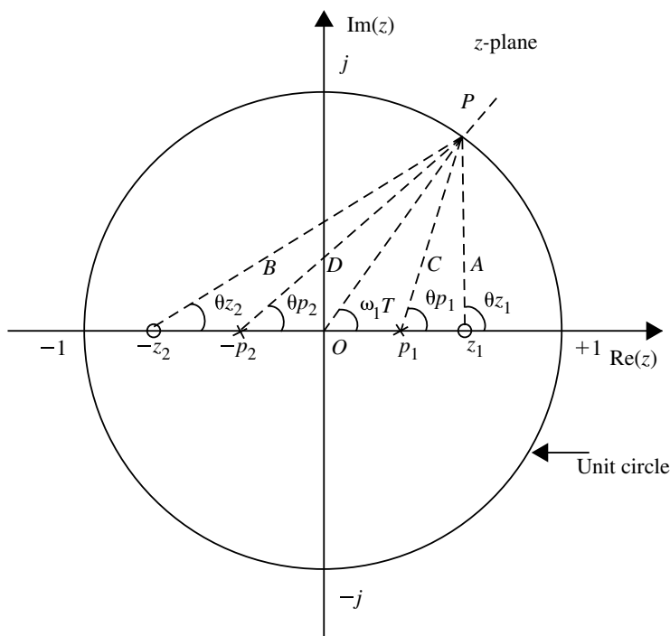
Fig. 4.26 Pole-zero diagram of H(z)
