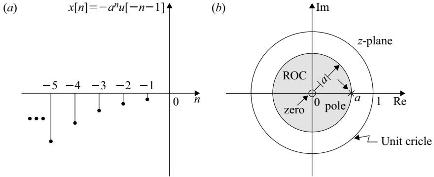
Fig. 2.3 a) x[n] = -a^n u[-n-1] and b) ROC: 0 < a < 1
