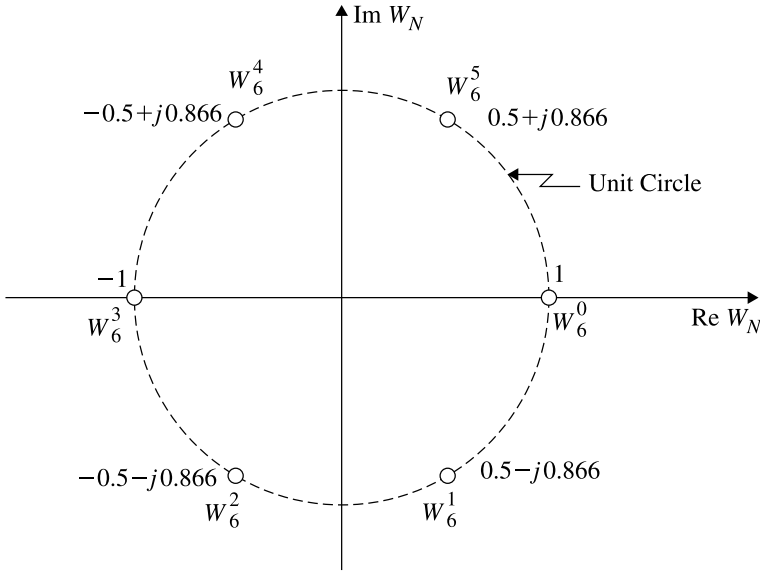
Fig. 3.2 Representation of W_6^{-nk}
