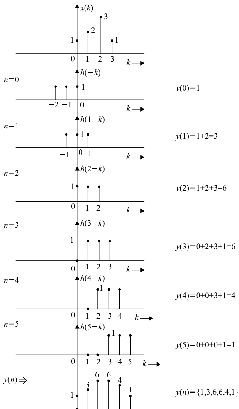
Fig. 3.12 Linear convolution of two sequences for Example 3.26
