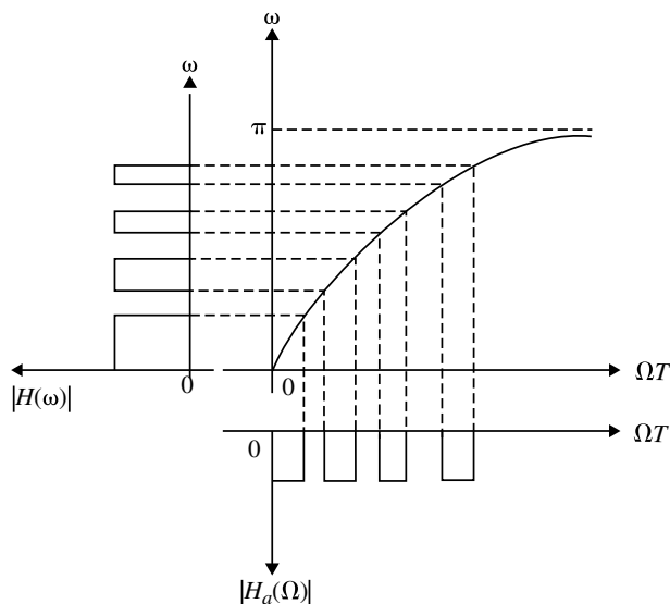
Fig. 4.6 Effect of warping on the magnitude response. (Equally spaced analog passbands are pushed together at high frequency in the digital domain.)
