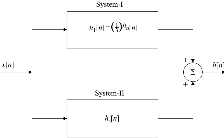
Fig. 2.23 Block diagram representation for Example 2.51
