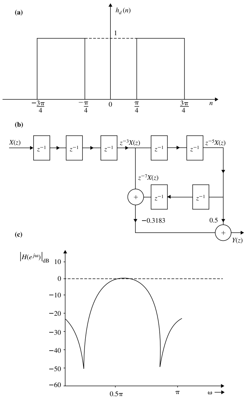
Fig. 5.28 a Impulse response for Example 5.11. b Structure realization for Example 5.11. c Frequency response of bandpass filter of Example 5.11
