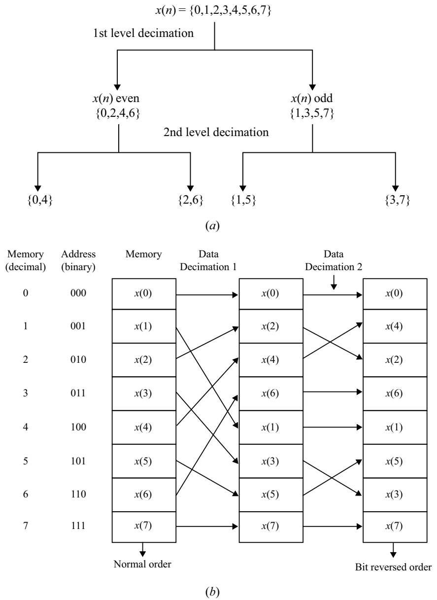
Fig. 3.14 a Data sequence decimation by radix-2. b Shifting of data and bit reversal
