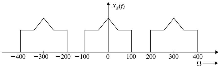
Fig. 1.67 Spectrum of sampled signal
