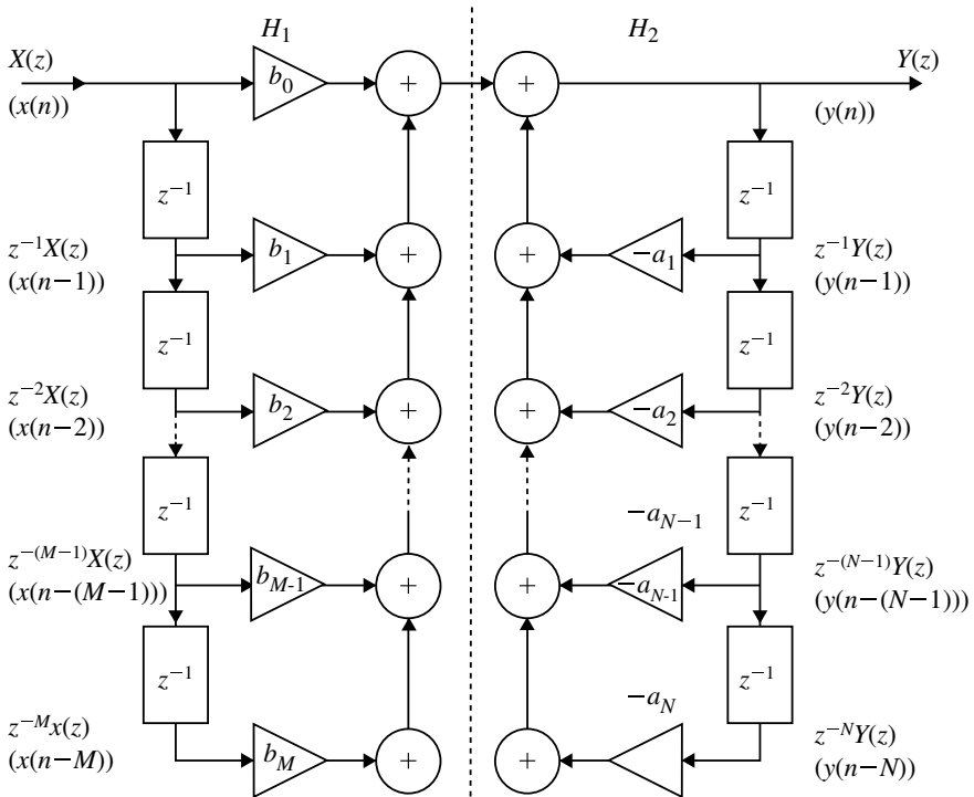
Fig. 4.29 Direct form-I realization
