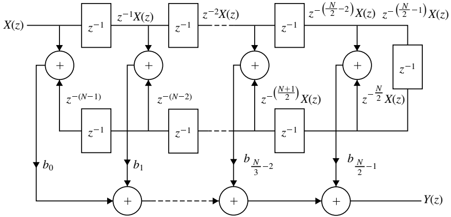
Fig. 5.4 Linear phase realization when N is even
