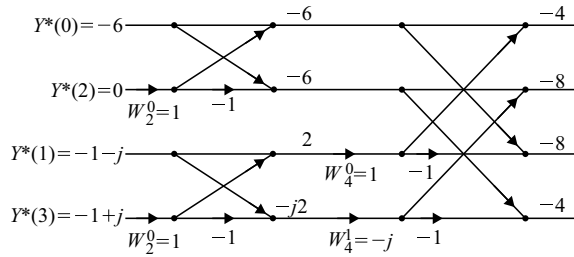
Fig. 3.28 Butterfly diagram of Y^*(k)
