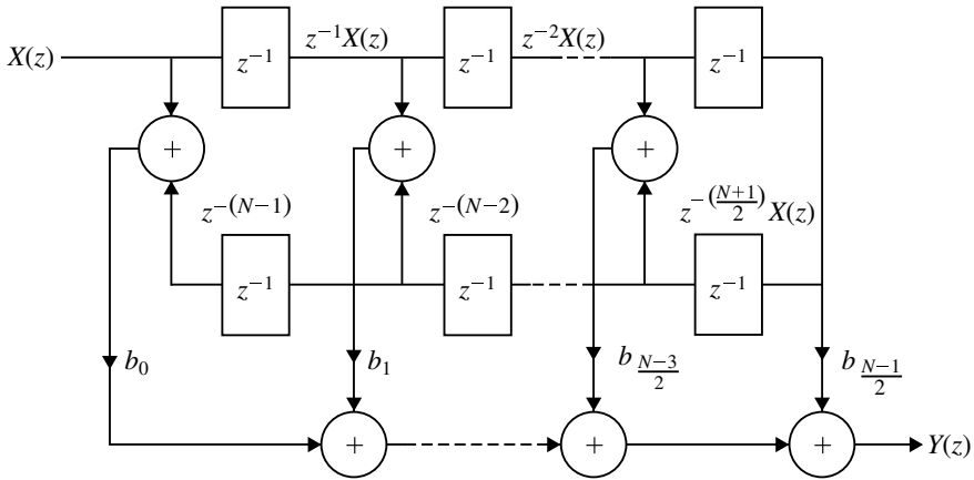
Fig. 5.5 Linear phase realization when N is odd
