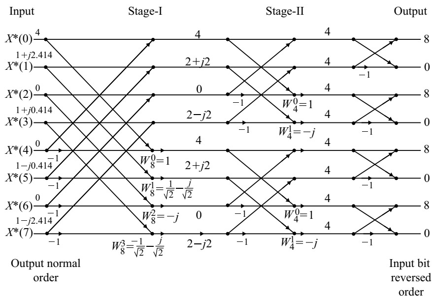
Fig. 3.32 Butterfly diagram of X^*(k)
