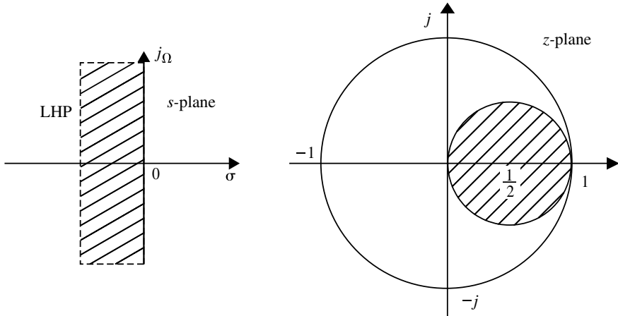
Fig. 4.25 The mapping from s -plane to z -plane by approximation of derivatives
