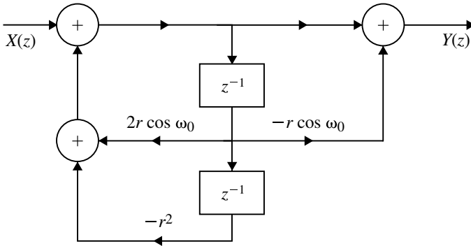
Fig. 4.38 Direct form-II realization for Example 4.31
