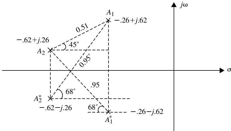
Fig. 4.16 Determination of residues by graphical method
