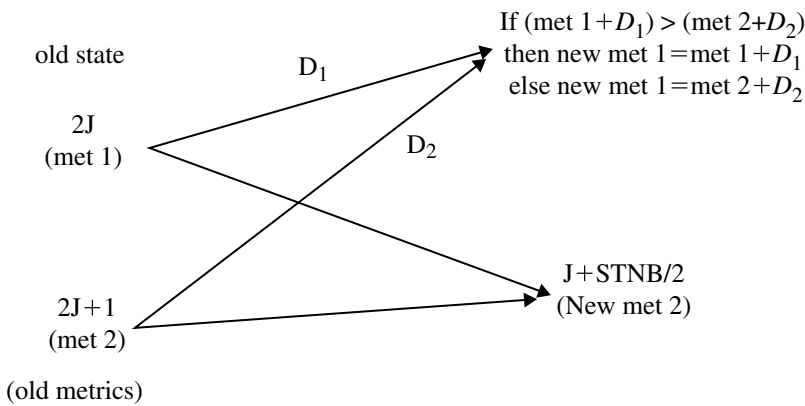
Fig. 6.15 Viterbi operator (STNB = no. of states, met path metrics and D = branch metrics)
