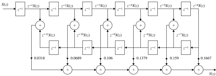
Fig. 5.48 Structure realization for Example 5.32
