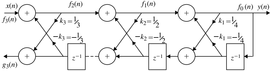
Fig. 4.61 Lattice structure for the Example 4.43
