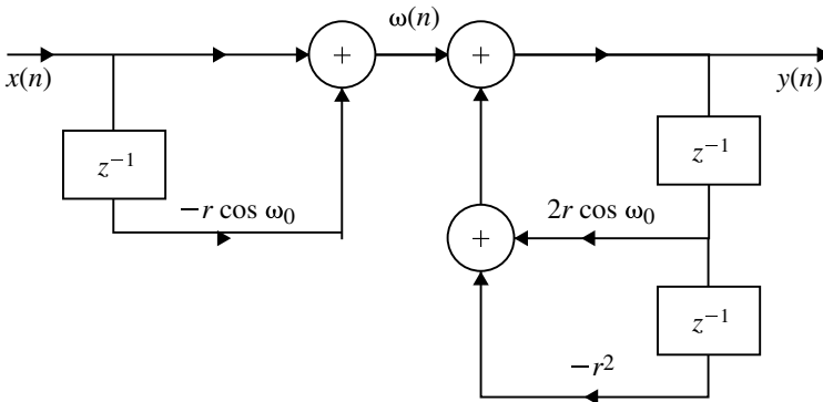
Fig. 4.36 Direct form-I realization for Example 4.29
