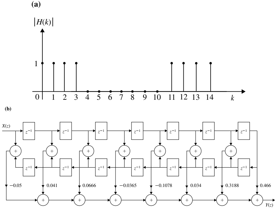
Fig. 5.47 a Ideal magnitude response for Example 5.31. b Structure realization for Example 5.31
