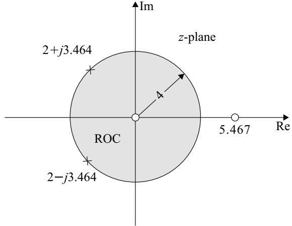
Fig. 2.11 Poles and zeros and ROC of Example 2.3.18
