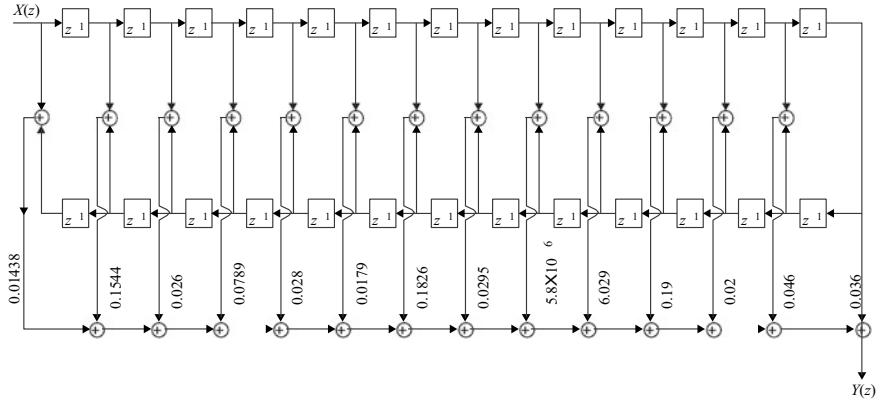
Fig. 5.39 Linear phase realization of H(z) for Example 5.17
