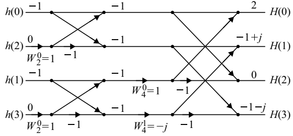
Fig. 3.27 Butterfly diagram of H(k)
