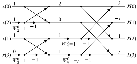
Fig. 3.26 Butterfly diagram of X(k)
