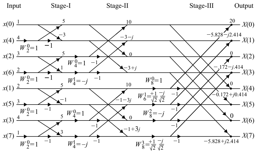
Fig. 3.29 Butterfly diagram of Example 3.33(i)
