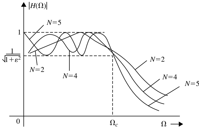
Fig. 4.23 Frequency response of Chebyshev filter type I filter
