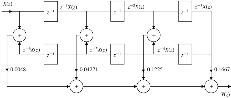
Fig. 5.46 FIR filter structure for Example 5.30
