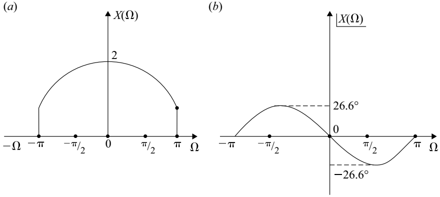
Fig. 2.22 Frequency spectra for Example 2.48. a Amplitude spectrum and b Phase spectrum
