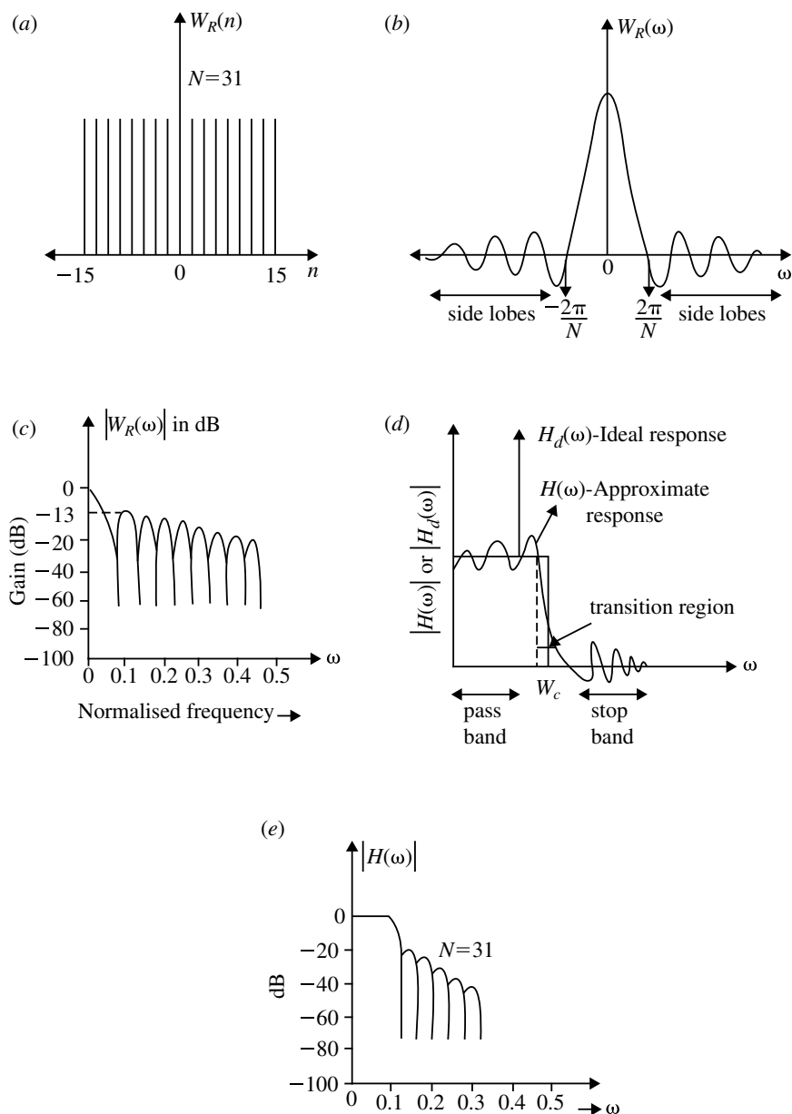
Fig. 5.30 Rectangular window sequence and its frequency response. a Rectangular window sequence; b Magnitude response of Rectangular window; c Log-magnitude response of Rectangular window; d Magnitude response of LPF approximated using Rectangular window and e Log-magnitude response of FIR LPF designed using Rectangular window
