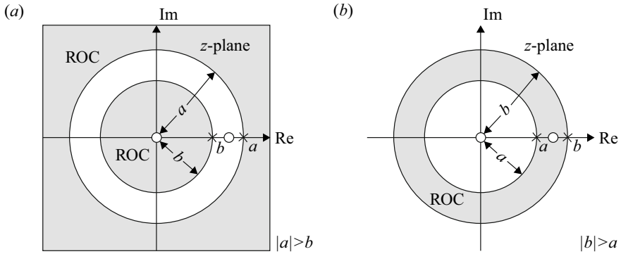
Fig. 2.4 ROC of a two-sided sequence
