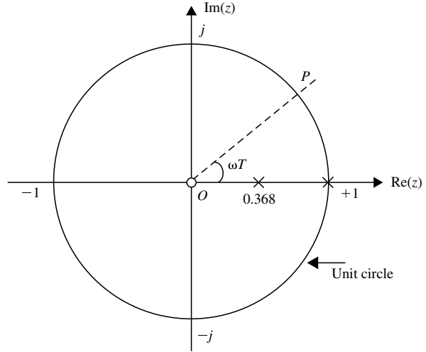
Fig. 4.27 Pole-zero diagram of Example 4.28
