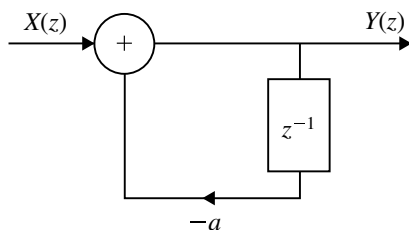
Fig. 5.51 Direct form realization for Problem 49
