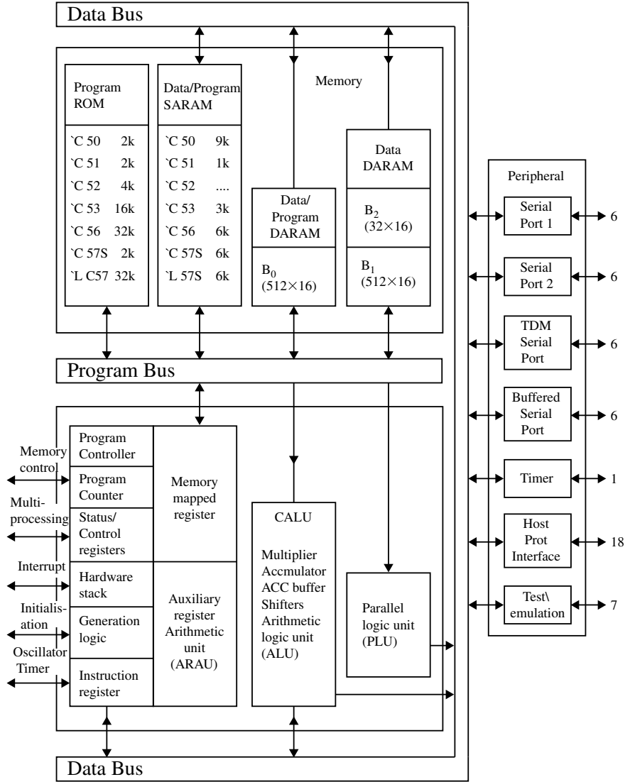
Fig. 6.9 Internal architecture of TMS320C5x
