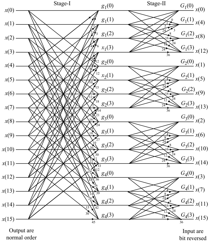
Fig. 3.20 16-Point radix-4 DIF FFT butterfly diagram
