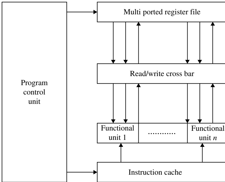
Fig. 6.6 Block diagram of the VLIW architecture
