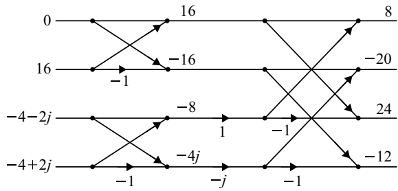
Fig. 3.53 Butterfly diagram of [X_2(k)H(k)]^*
