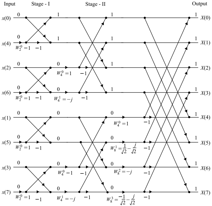
Fig. 3.36 Butterfly diagram for Example 3.39
