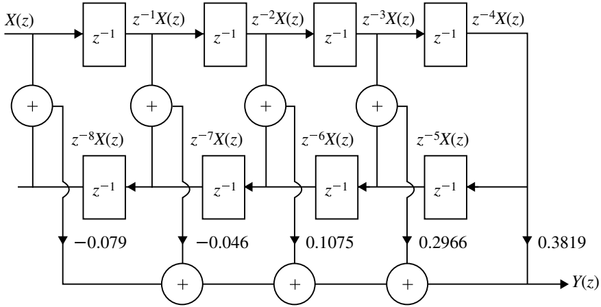
Fig. 5.31 Linear phase realization of H(z) for Example 5.13
