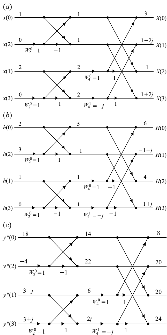
Fig. 3.39 a Butterfly diagram for Example 3.42. b Butterfly diagram for Example 3.42. c Butterfly diagram for Example 3.42
