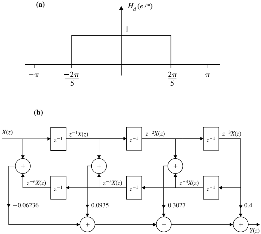
Fig. 5.43 a Frequency Response of for Example 5.27. b Linear phase realization of FIR filter for Example 5.27
