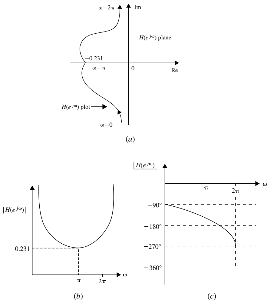
Fig. 4.28 a Frequency response polar plot of discrete system. b Magnitude response. c Phase response
