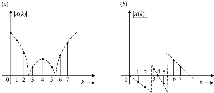
Fig. 3.8 Magnitude and phase spectrum for N = 8
