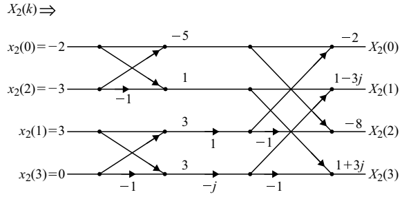
Fig. 3.52 Butterfly diagram of X_2(k)
