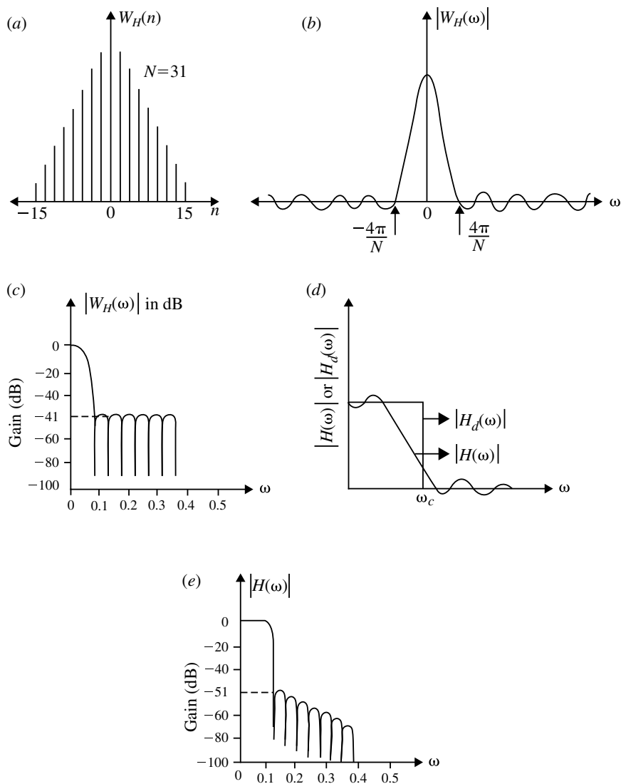
Fig. 5.34 Hamming window sequence and its frequency response. a Hamming window sequence; b Magnitude response of Hamming window; c Log-magnitude response of Hamming window; d Magnitude response of LPF approximated using Hamming window and e Log-magnitude response of FIR filter using Hamming window
