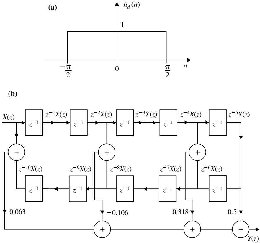
Fig. 5.26 a Impulse response of LPF for Example 5.9. b Structure realization for Example 5.9
