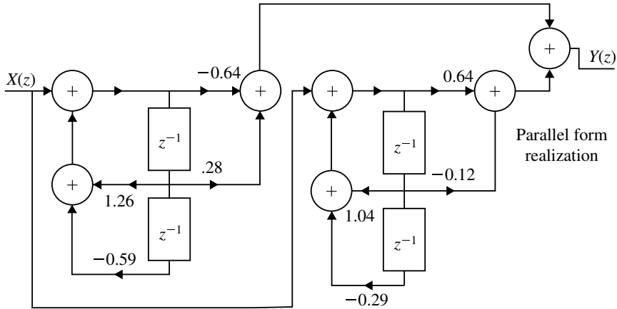
Fig. 4.17 Parallel form realization of H(z) for Example 4.9
