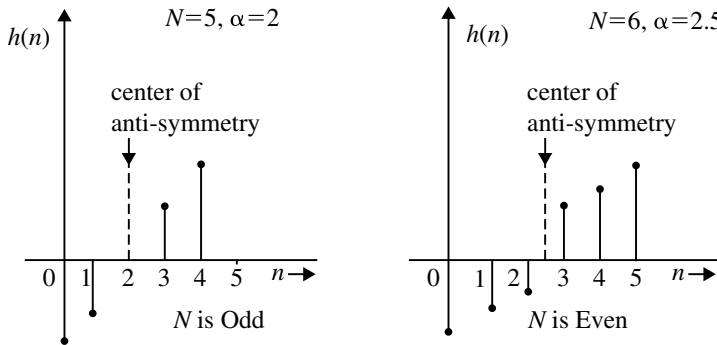
Fig. 5.18 Anti-symmetry impulse response for N = \text{odd} and N = \text{even}
