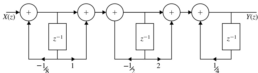
Fig. 4.48 Cascade form realization of H(z) for the Example 4.37
