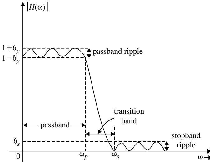
Fig. 5.2 Magnitude response of a practical lowpass filter
