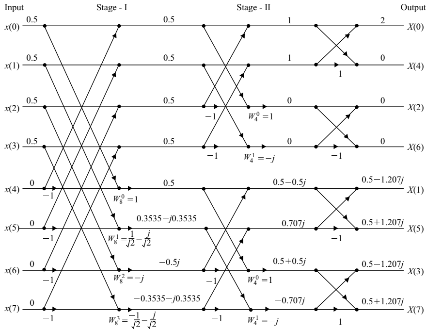
Fig. 3.37 Butterfly diagram for Example 3.40
