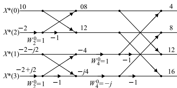
Fig. 3.33 Butterfly diagram of X^*(k)
