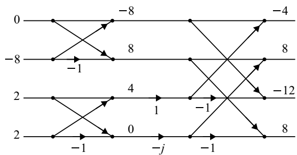
Fig. 3.51 Butterfly diagram of [X_1(k)H(k)]^*
