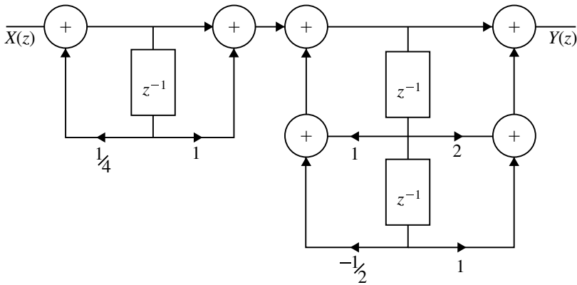
Fig. 4.52 Cascade form realization of H(z) for the Example 4.39
