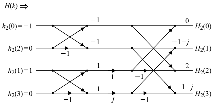
Fig. 3.57 Butterfly diagram of H(k)
