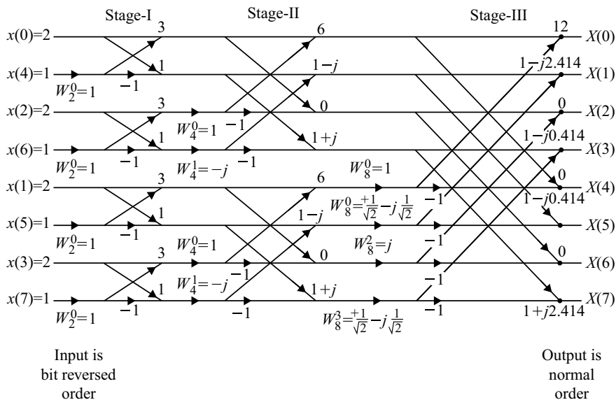
Fig. 3.23 Butterfly diagram of Example 3.31(i)
