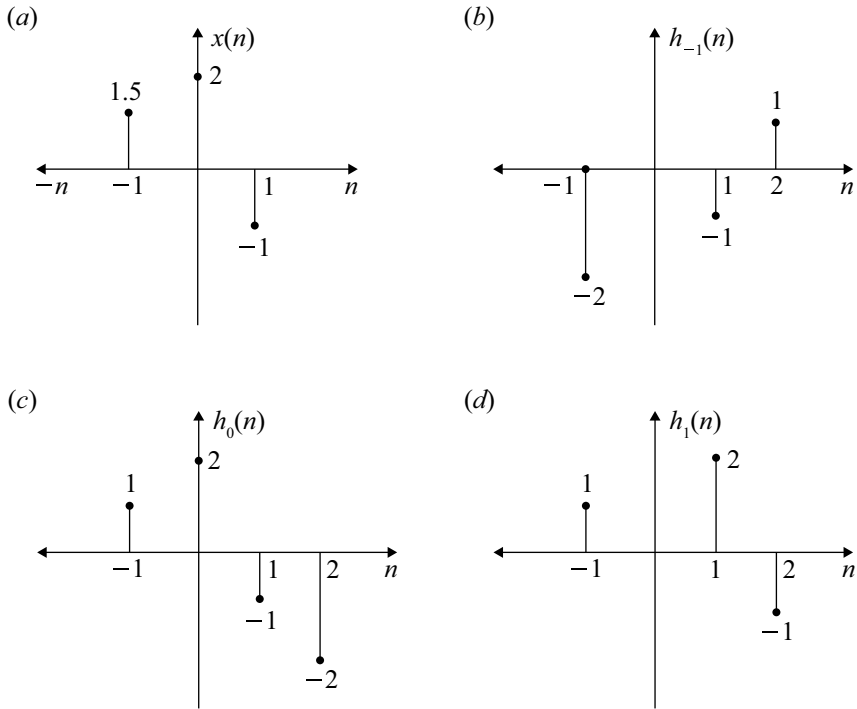
Fig. 2.24 Input and impulse response sequences
