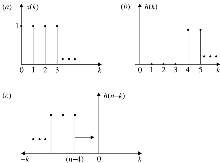
Fig. 2.32 Signals of Example 2.63
