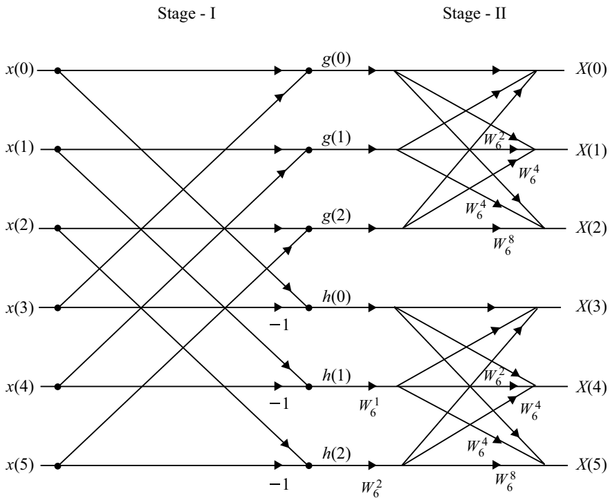
Fig. 3.46 DIF FFT flow diagram for decomposing the DFT for N = 6 = 3 \cdot 2
