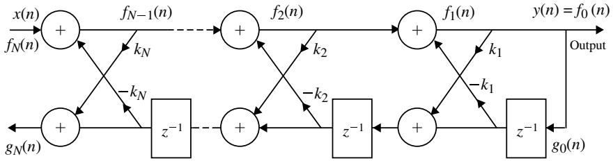
Fig. 4.58 All-pole lattice filter
