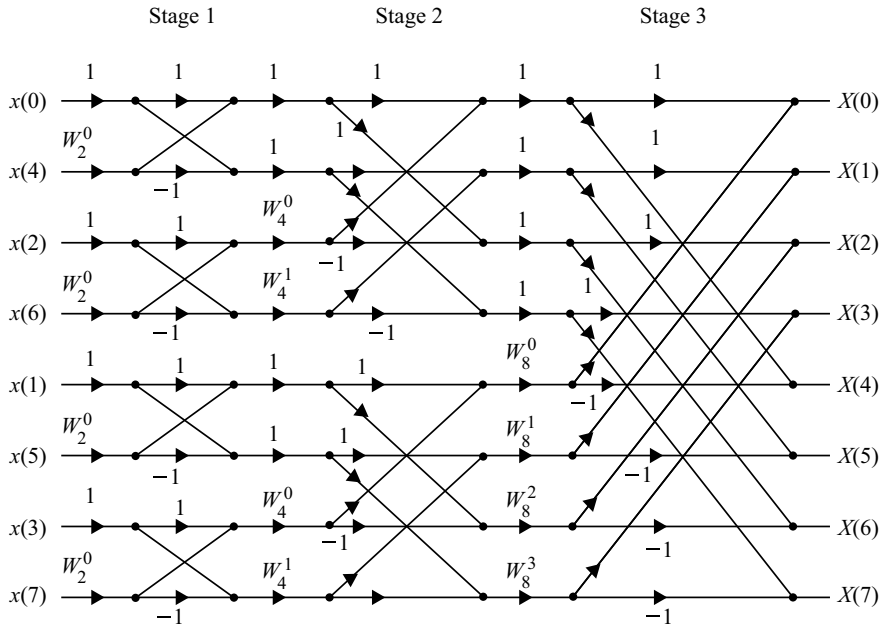
Fig. 3.17 8-point radix-2 DIT FFT Butterfly diagram
