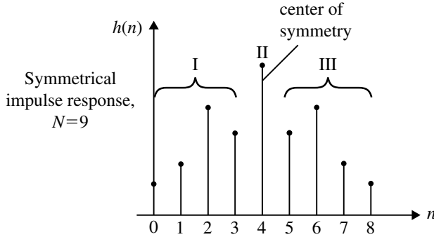
Fig. 5.19 Symmetry impulse response when N = \text{odd}
