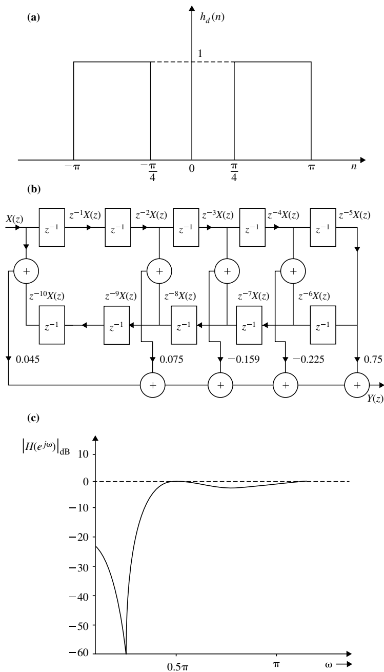
Fig. 5.27 a Impulse response for Example 5.10. b Structure realization for Example 5.10. c Magnitude response for Example 5.10
