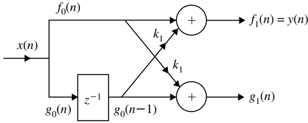
Fig. 5.13 Single-stage all-zero lattice structure
