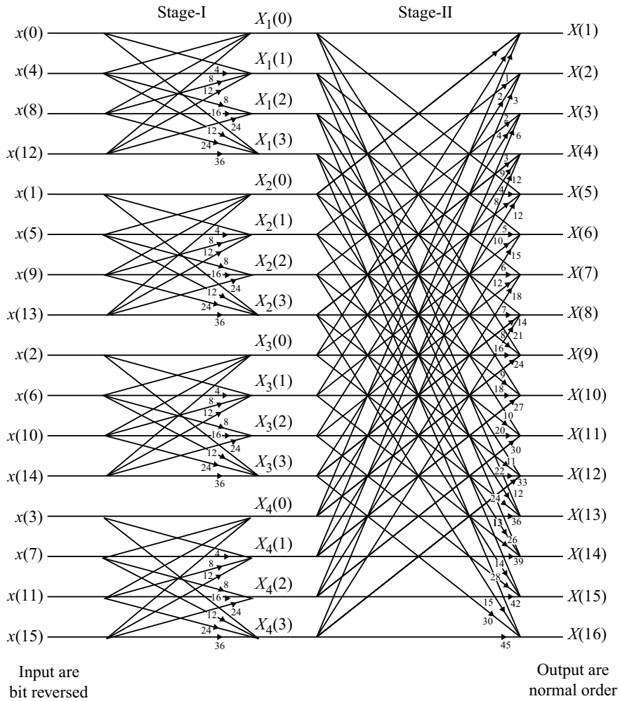
Fig. 3.19 16-Point radix-4 DIT FFT butterfly diagram
