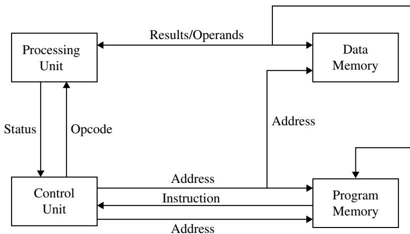
Fig. 6.4 Modified Harvard architecture
