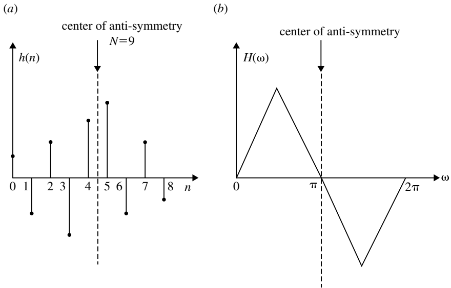
Fig. 5.23 a Anti-symmetric impulse response for N = 9 . b Magnitude function of H(\omega)
