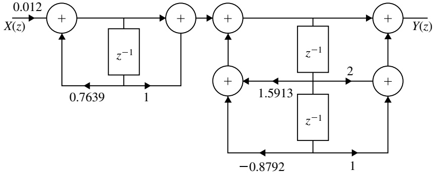
Fig. 4.24 Cascade form realization of H(z) for the Example 4.22
