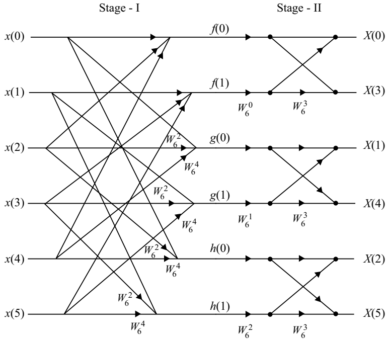
Fig. 3.47 DIF FFT flow diagram for decomposing the DFT for N = 6 = 2 \cdot 3
