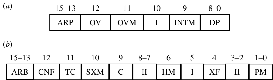
Fig. 6.10 a Status register (ST0) bit assignment and b status register (ST1) bit assignment
