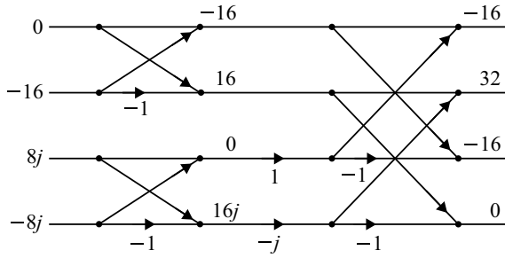
Fig. 3.62 DFT Computation of [X_3(k)H(k)]^*
