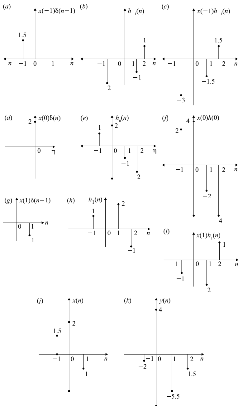
Fig. 2.25 Convolution sum of discrete signals
