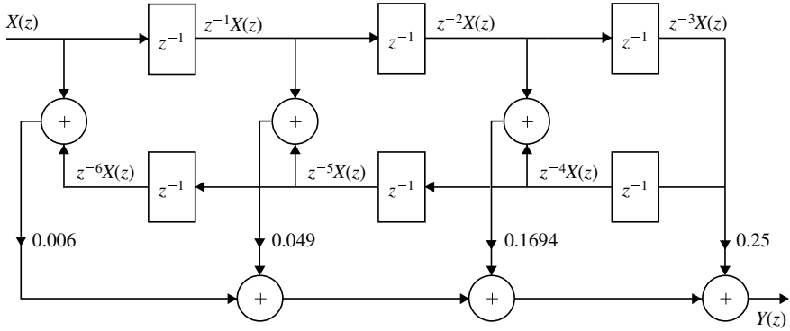
Fig. 5.49 Structure realization for Example 5.34
