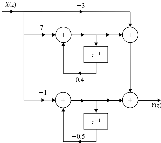
Fig. 4.43 Parallel form realization for Example 4.34
