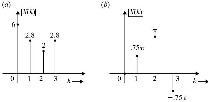
Fig. 3.5 Magnitude and phase spectrum of Example 3.8
