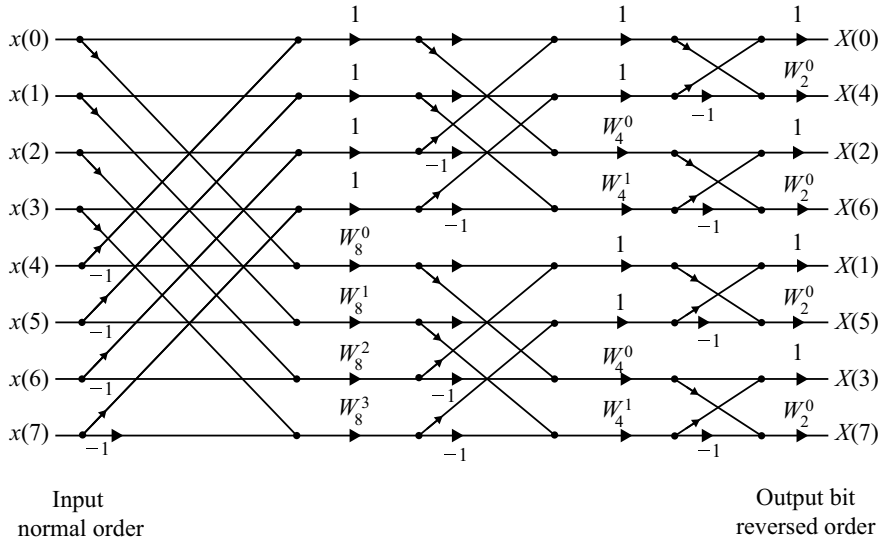
Fig. 3.18 8-point radix-2 DIF-FFT butterfly diagram
