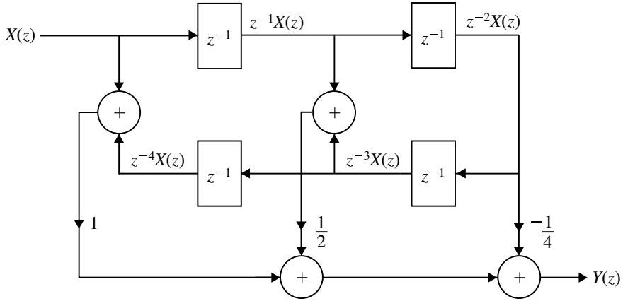
Fig. 5.45 Linear Phase Realization for Example 5.29
