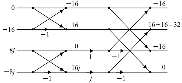
Fig. 3.55 Butterfly diagram of [x_3(k)H(k)]^*
