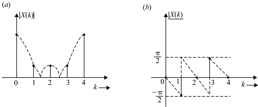
Fig. 3.4 Magnitude and phase spectrum of Example 3.7
