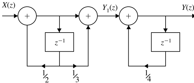
Fig. 4.40 Cascade form realization for Example 4.33
