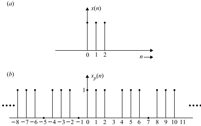
Fig. 3.6 DT signal and its periodic extension
