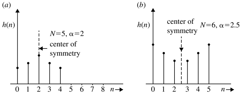
Fig. 5.17 Symmetry impulse response for N = \text{odd} and N = \text{even}
