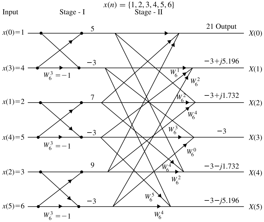
Fig. 3.43 Butterfly diagram for Example 3.44(c)
