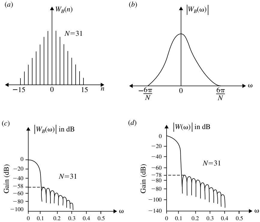
Fig. 5.36 Blackman window sequence and its frequency response. a Blackman window sequence; b Magnitude response of Blackman window; c Log-magnitude response of Blackman window and d Log-magnitude response of FIR LPF approximated using Blackman window
