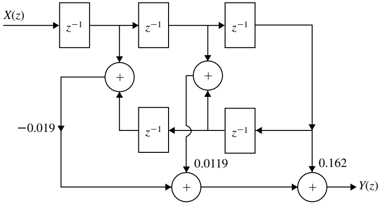
Fig. 5.37 Linear phase realization of H(z) for Example 5.16
