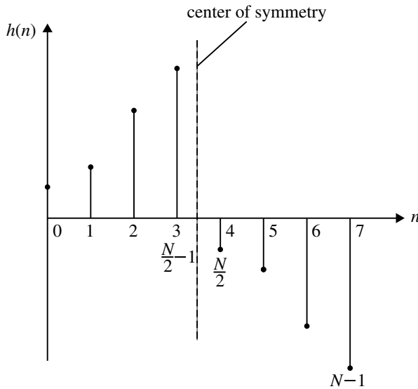
Fig. 5.24 Anti-symmetric impulse response for N = \text{even}
