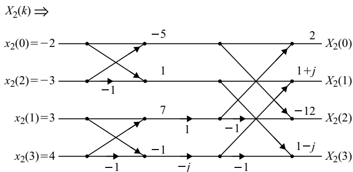
Fig. 3.59 DFT Computation of X_2(k)
