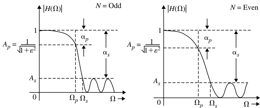
Fig. 4.22 Frequency response of type II Chebyshev filter. a N is odd and b N is even
