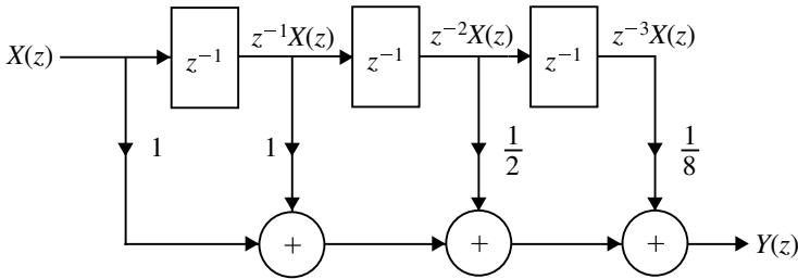
Fig. 5.7 Direct form realization of FIR filter for Example 5.2
