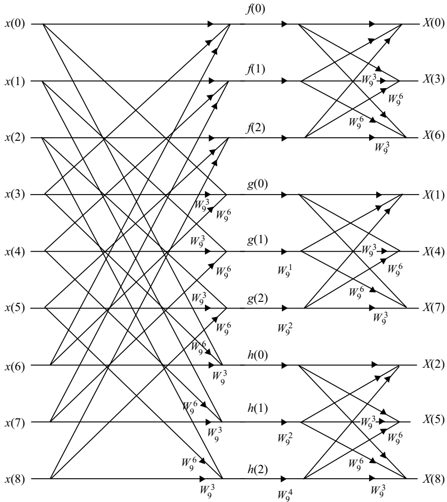
Fig. 3.48 A radix-3 DIF FFT flow diagram for decomposing the DFT for N = 9 = 3 \cdot 3
