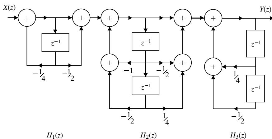
Fig. 4.45 Cascade form realization for Example 4.36
