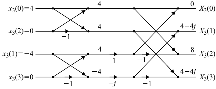
Fig. 3.54 Butterfly diagram of X_3(k)
