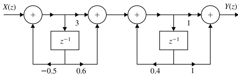
Fig. 4.42 Cascade form realization for Example 4.34
