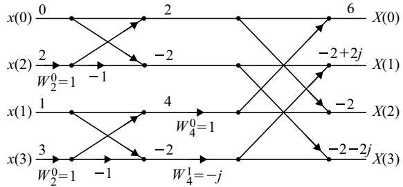
Fig. 3.31 Butterfly diagram of X(k) for Example 3.34
