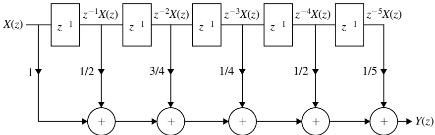
Fig. 5.6 Direct form (or) transversal realization of H(z) for Example 5.1
