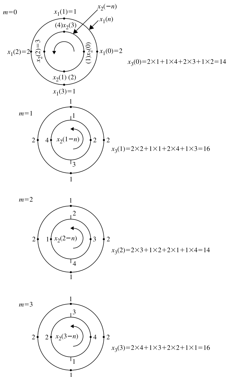
Fig. 3.11 Circular convolution of Example 3.22 for different values of m
