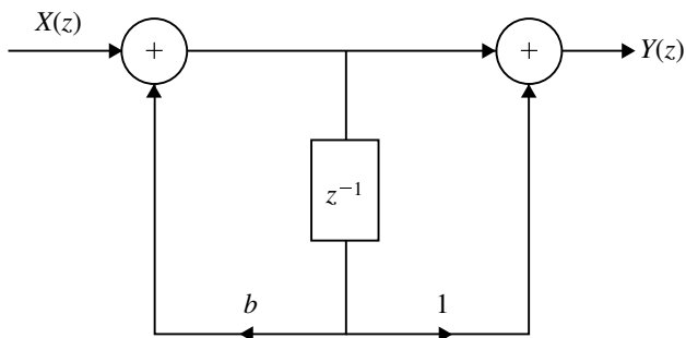
Fig. 5.52 A structure for Problem 50
