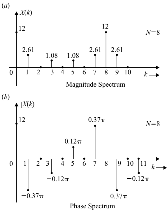
Fig. 3.25 Magnitude and phase spectrum of Example 3.31
