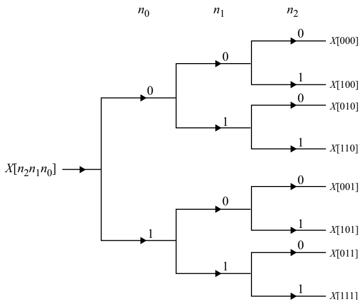
Fig. 3.65 Tree diagram depicting bit reversed-order sorting
