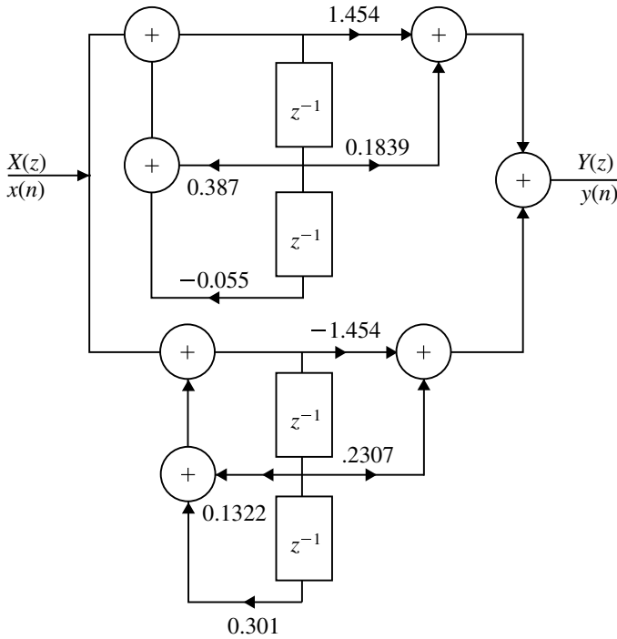
Fig. 4.19 Parallel form realization of H(z) for Example 4.10
