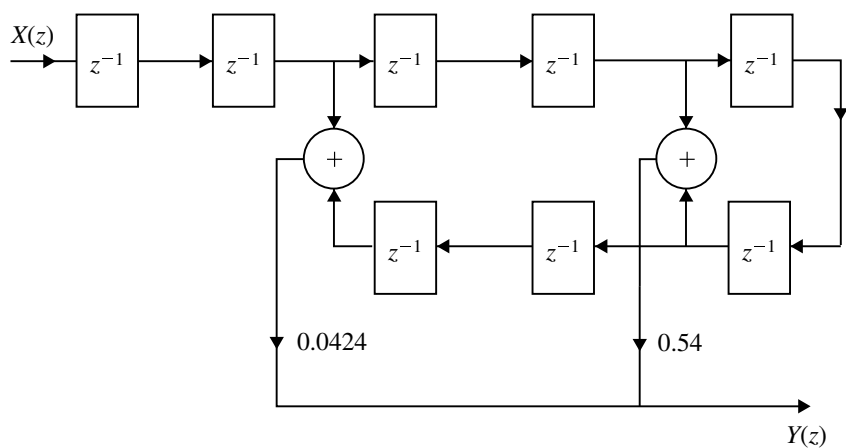
Fig. 5.42 a Structure realization (rectangular window) for Example 5.26. b Structure realization (Blackman window) for Example 5.26
