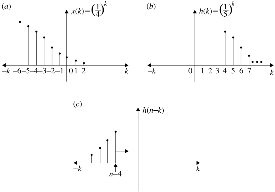
Fig. 2.30 Representation of signals for Example 2.61
