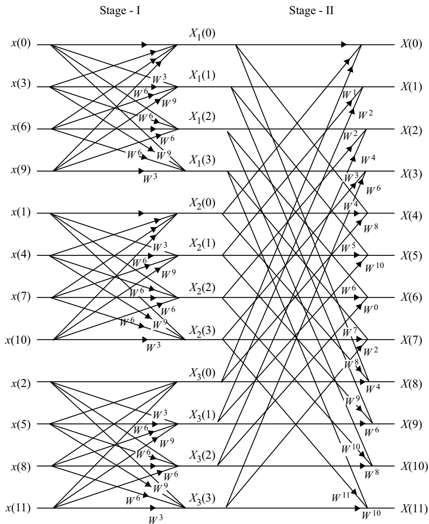
Fig. 3.44 Flow diagram of 12-point composite radix-FFT
