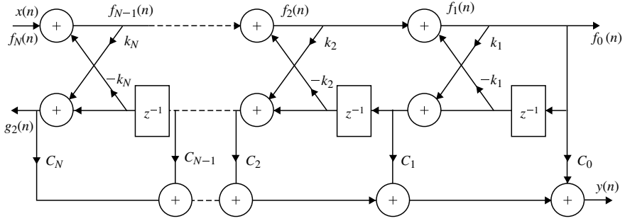
Fig. 4.59 Lattice-ladder structure for realizing a pole-zero IIR filter
