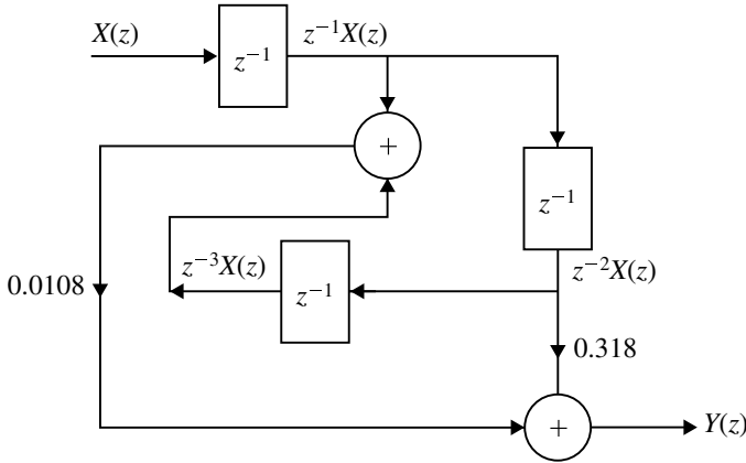
Fig. 5.33 Linear phase realization of H(z) for Example 5.14
