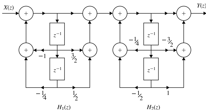
Fig. 4.44 Cascade form realization for Example 4.35
