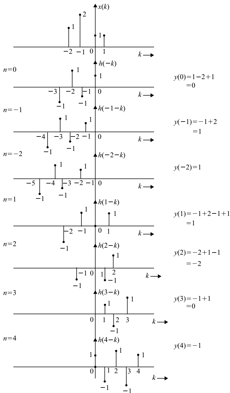
Fig. 3.13 Linear convolution of two sequences for Example 3.30
