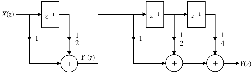
Fig. 5.8 Cascade form realization of FIR filter for Example 5.2
