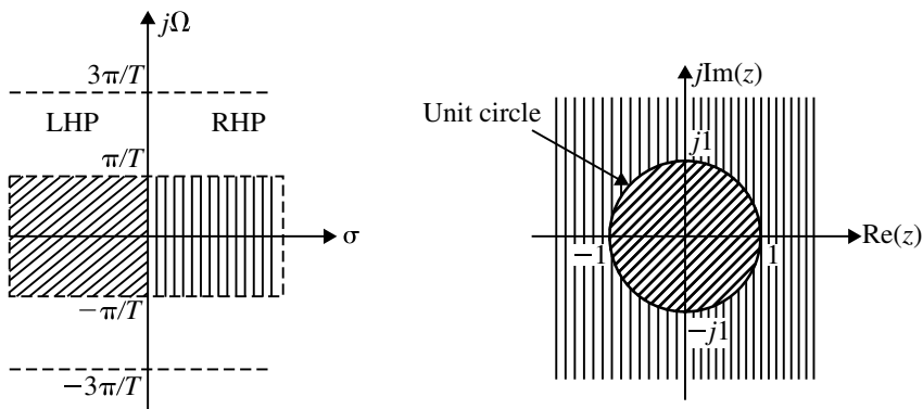
Fig. 4.62 Mapping of s -plane into z -plane in impulse invariant transformation
