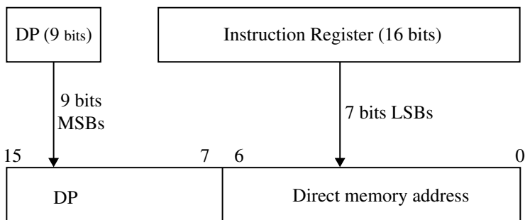
Fig. 6.11 16-bit data memory address bus
