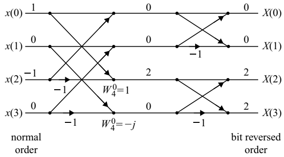
Fig. 3.34 Butterfly diagram of X(k) for Example 3.37
