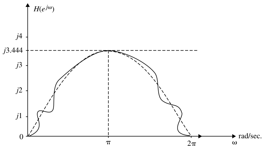
Fig. 5.41 a Structure realization (rectangular window) for Example 5.25. b Frequency response plot. c Structure realization (Hamming window) for Example 5.25. d
