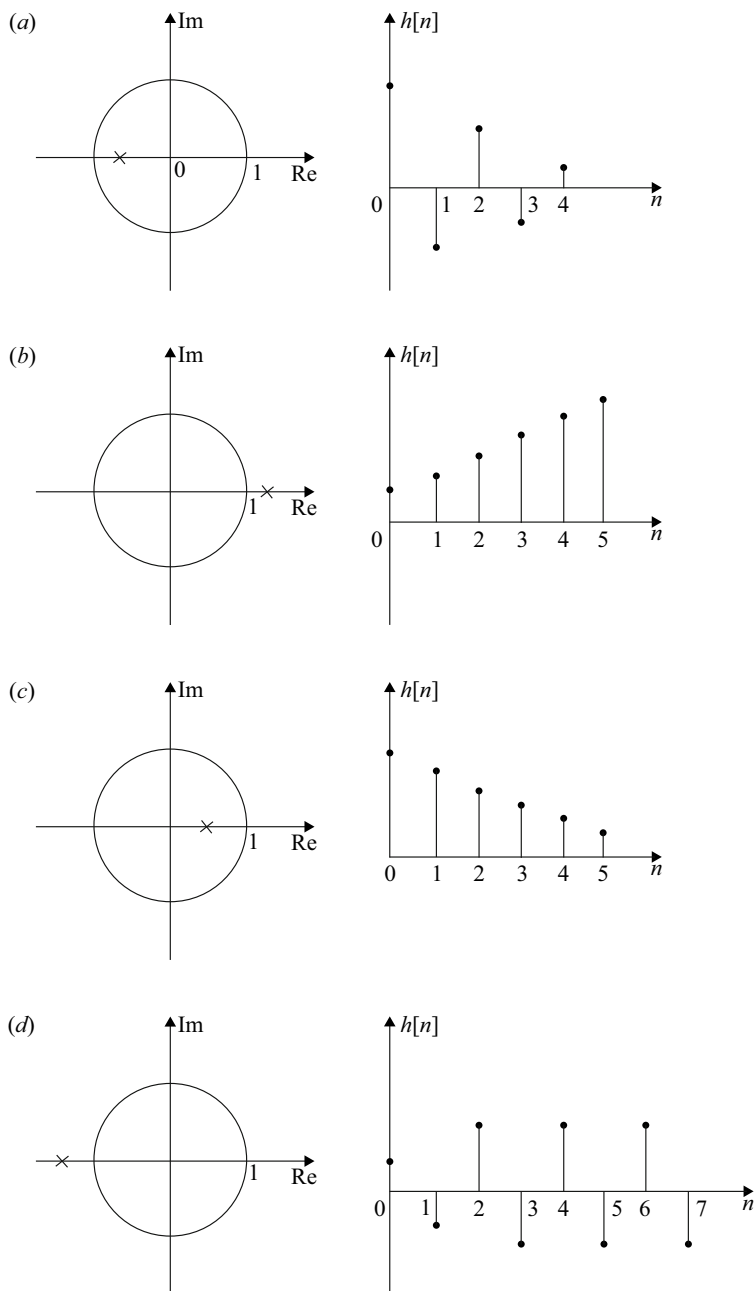
Fig. 2.15 a to d Pole location and impulse response of a causal system. e to f Pole location and impulse response of a causal system
