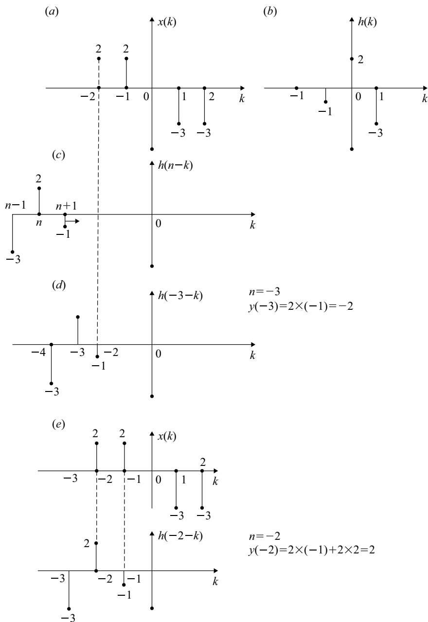
Fig. 2.35 Graphical method of obtaining y(n] of Example 2.70(a) to (e). Graphical method of obtaining y(n] of Example 2.70(f) to (k)
