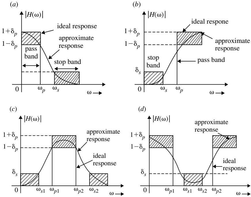
Fig. 4.2 Magnitude response. a Lowpass, b Highpass, c Bandpass and d Band stop filter
