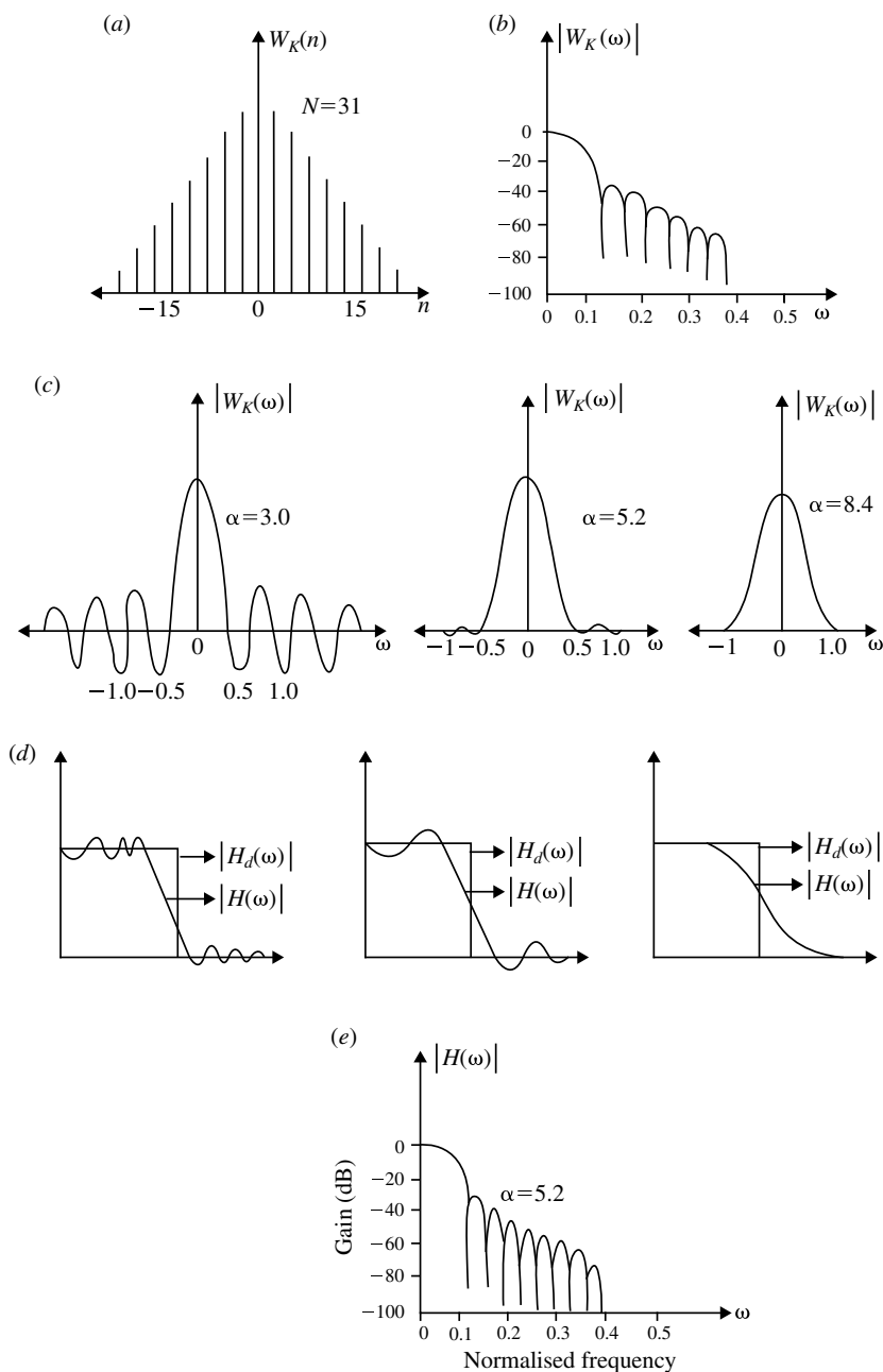
Fig. 5.38 Kaiser window sequence and its frequency response. a Kaiser window sequence; b Log-magnitude response of Kaiser window; c Magnitude frequency response of Kaiser window for different values of \alpha (when N = 31 ); d Magnitude response of Kaiser window for different values of \alpha (when N = 31 ) and e Log-magnitude response of FIR LPF designed using Kaiser window
