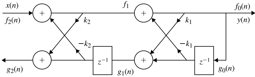
Fig. 4.57 Two stage all-pole lattice filter
