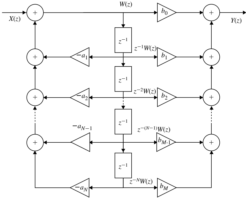
Fig. 4.30 Direct form-II structure of IIR system for N = M
