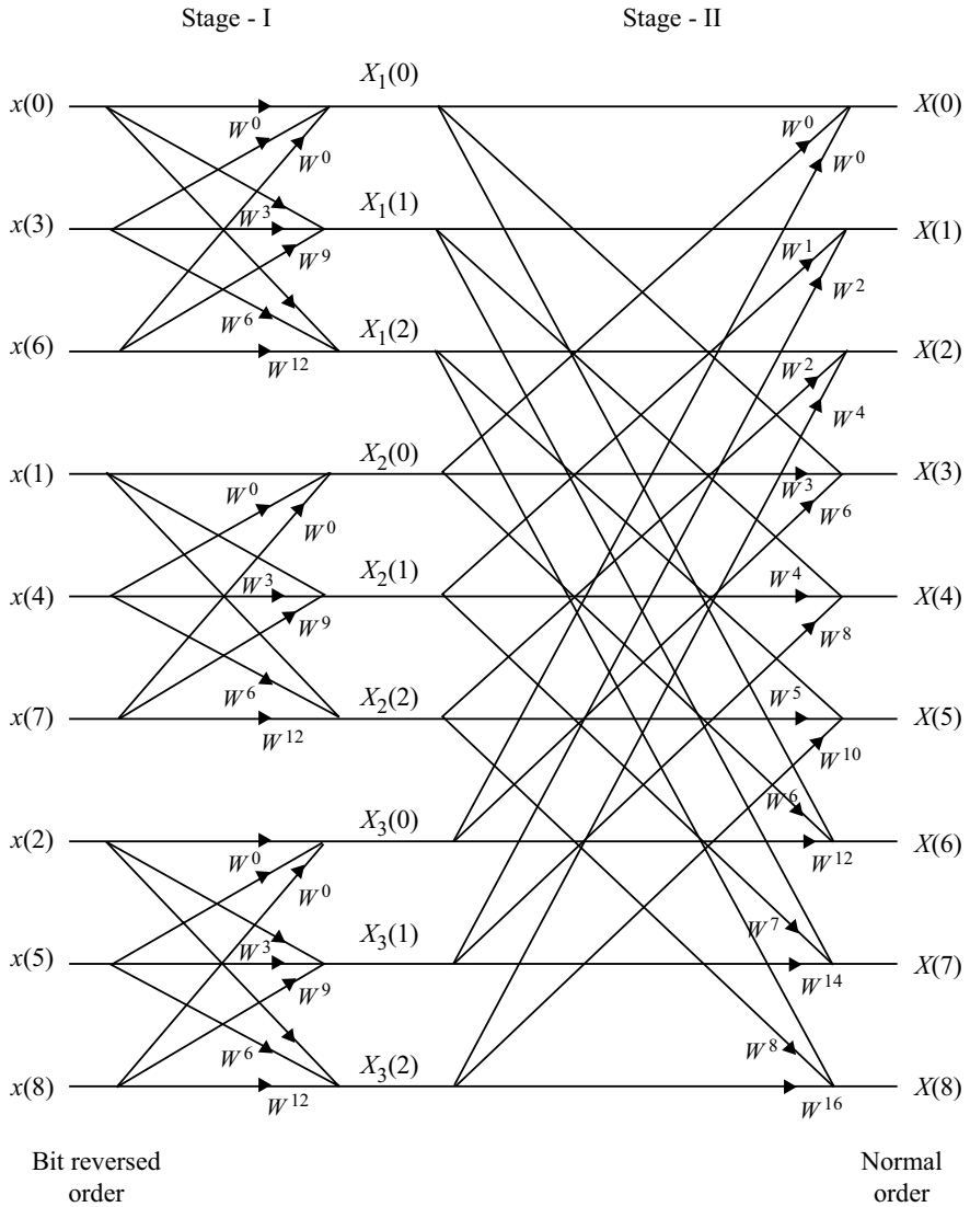
Fig. 3.40 Radix-3 DIT FFT flow diagram for N = 9
