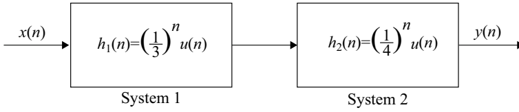
Fig. 2.28 Impulse response of two systems connected in cascade
