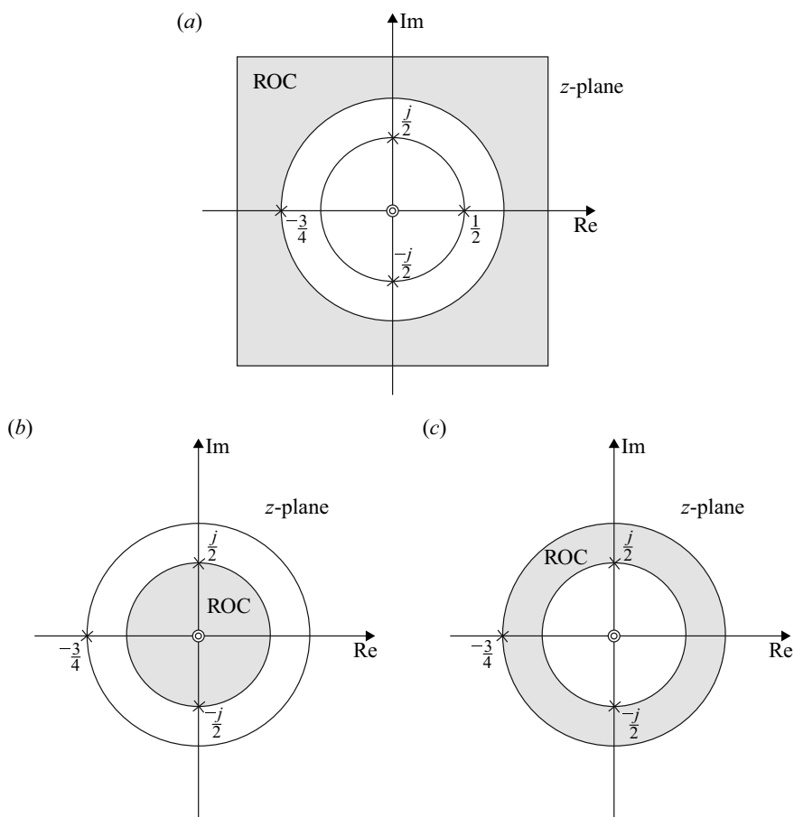
Fig. 2.12 Pole-zero diagram and ROC of X[z]
