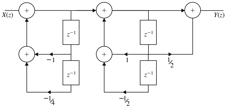
Fig. 4.50 Cascade form realization of H(z) for the Example 4.38
