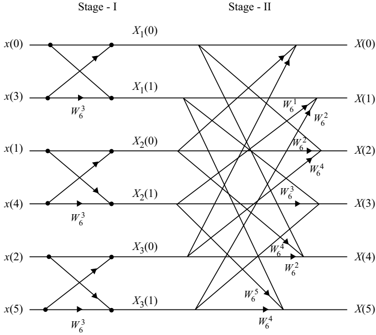
Fig. 3.42 DIT FFT flow diagram for N = 6 = 3 \cdot 2
